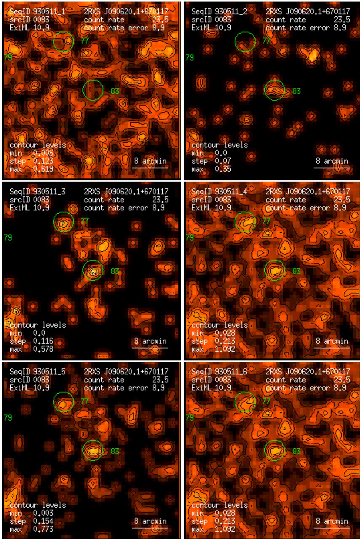
Figure 83: RASS 930511: detection 0083: band rate images, Gaussian filter: (1) PSPC channels 11 – 41, (2) 52 – 90, (3) 91 – 201, (4) 11 – 235, (5) 52 – 201, (6) 11 – 201. Broad band rates in counts/ks. Band rate contour levels in counts/ks/arcmin 2 .
