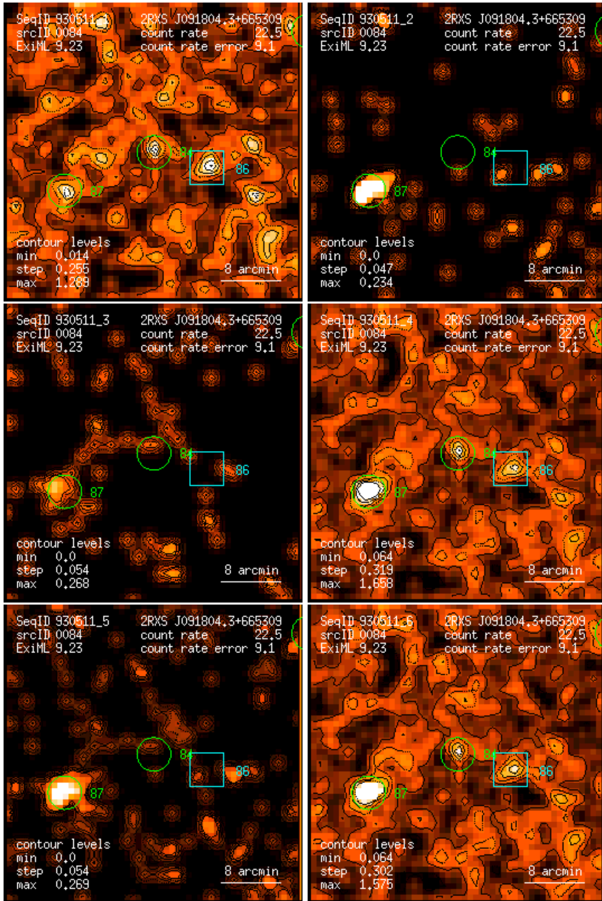
Figure 84: RASS 930511: detection 0084: band rate images, Gaussian filter: (1) PSPC channels 11 – 41, (2) 52 – 90, (3) 91 – 201, (4) 11 – 235, (5) 52 – 201, (6) 11 – 201. Broad band rates in counts/ks. Band rate contour levels in counts/ks/arcmin 2 .
