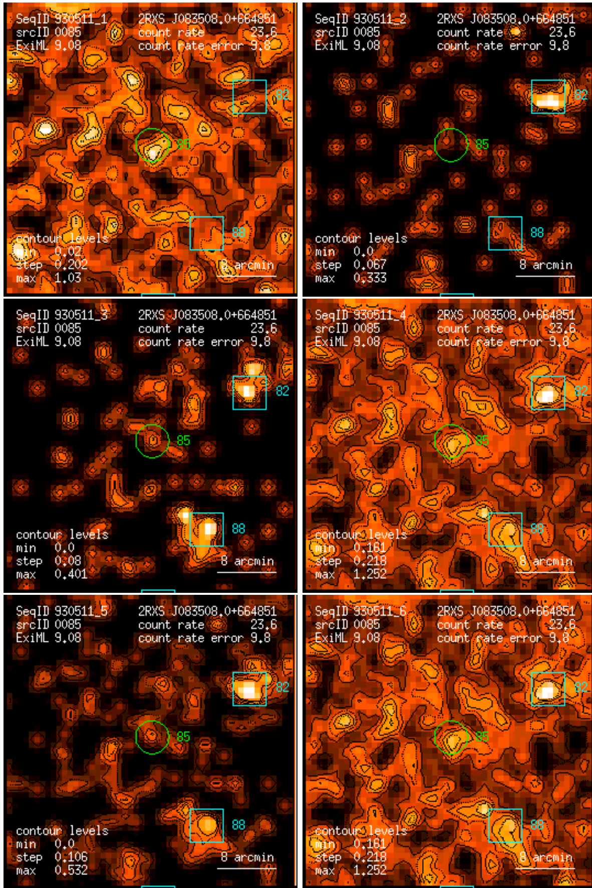
Figure 85: RASS 930511: detection 0085: band rate images, Gaussian filter: (1) PSPC channels 11 – 41, (2) 52 – 90, (3) 91 – 201, (4) 11 – 235, (5) 52 – 201, (6) 11 – 201. Broad band rates in counts/ks. Band rate contour levels in counts/ks/arcmin 2 .
