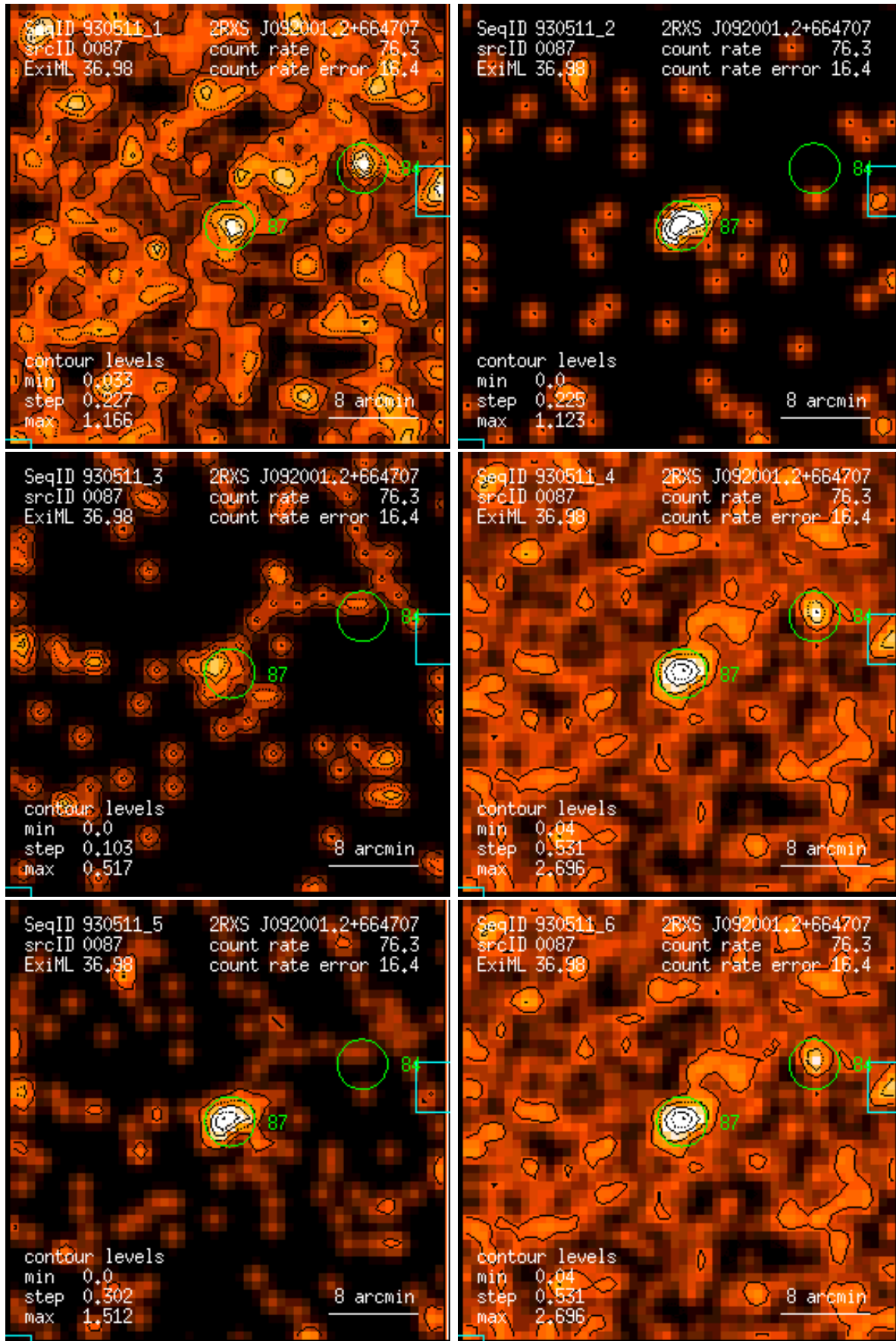
Figure 87: RASS 930511: detection 0087: band rate images, Gaussian filter: (1) PSPC channels 11 – 41, (2) 52 – 90, (3) 91 – 201, (4) 11 – 235, (5) 52 – 201, (6) 11 – 201. Broad band rates in counts/ks. Band rate contour levels in counts/ks/arcmin 2 .
