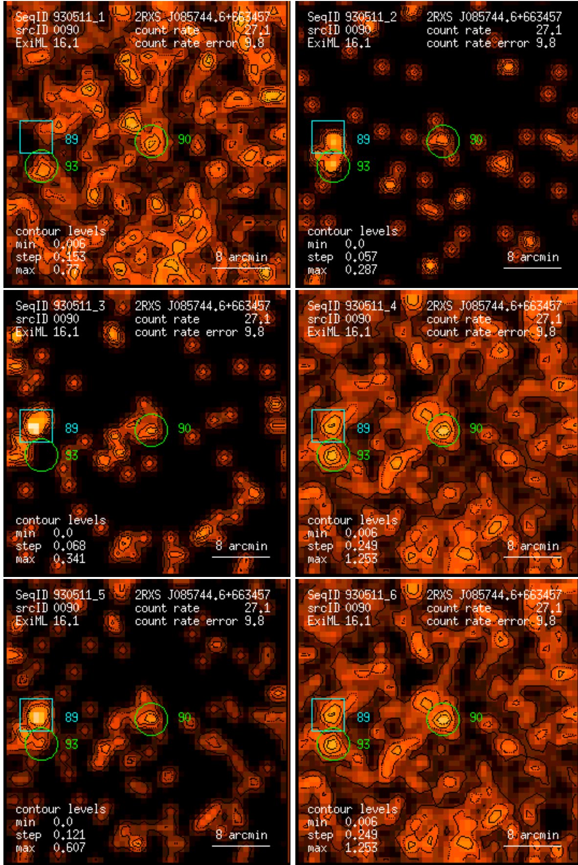
Figure 90: RASS 930511: detection 0090: band rate images, Gaussian filter: (1) PSPC channels 11 – 41, (2) 52 – 90, (3) 91 – 201, (4) 11 – 235, (5) 52 – 201, (6) 11 – 201. Broad band rates in counts/ks. Band rate contour levels in counts/ks/arcmin 2 .
