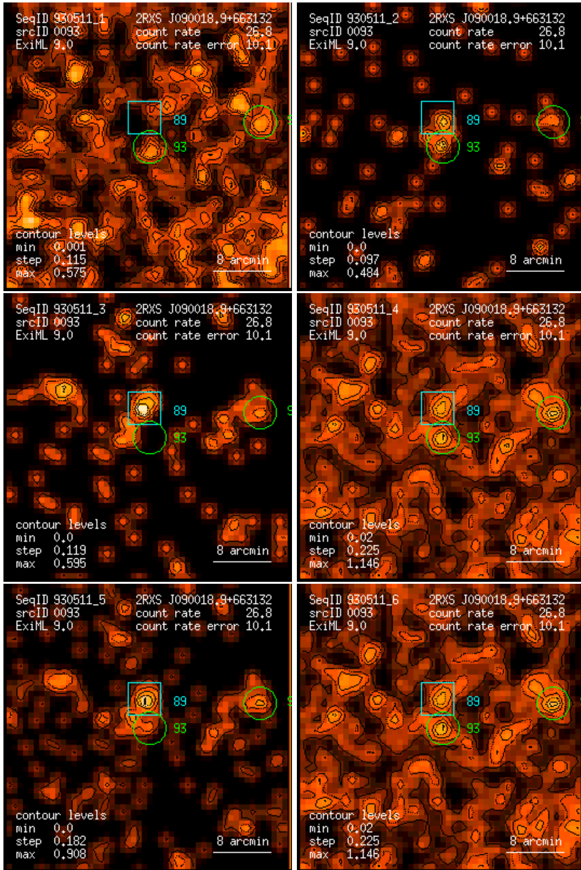
Figure 93: RASS 930511: detection 0093: band rate images, Gaussian filter: (1) PSPC channels 11 – 41, (2) 52 – 90, (3) 91 – 201, (4) 11 – 235, (5) 52 – 201, (6) 11 – 201. Broad band rates in counts/ks. Band rate contour levels in counts/ks/arcmin 2 .
