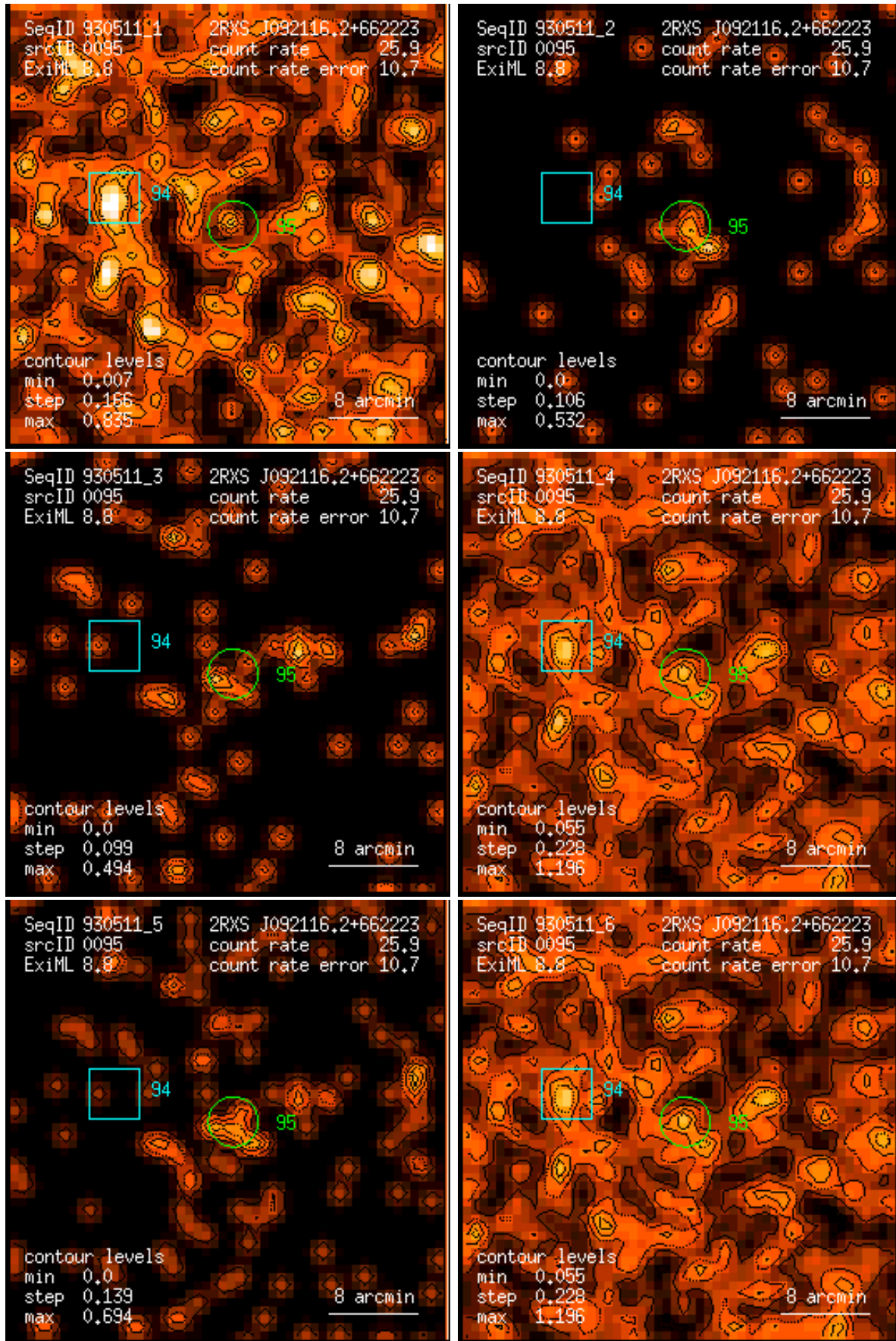
Figure 95: RASS 930511: detection 0095: band rate images, Gaussian filter: (1) PSPC channels 11 – 41, (2) 52 – 90, (3) 91 – 201, (4) 11 – 235, (5) 52 – 201, (6) 11 – 201. Broad band rates in counts/ks. Band rate contour levels in counts/ks/arcmin 2 .
