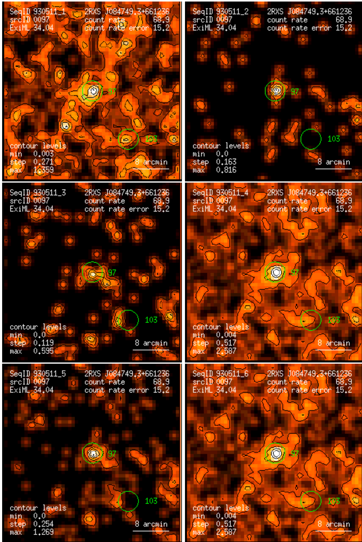
Figure 97: RASS 930511: detection 0097: band rate images, Gaussian filter: (1) PSPC channels 11 – 41, (2) 52 – 90, (3) 91 – 201, (4) 11 – 235, (5) 52 – 201, (6) 11 – 201. Broad band rates in counts/ks. Band rate contour levels in counts/ks/arcmin 2 .
