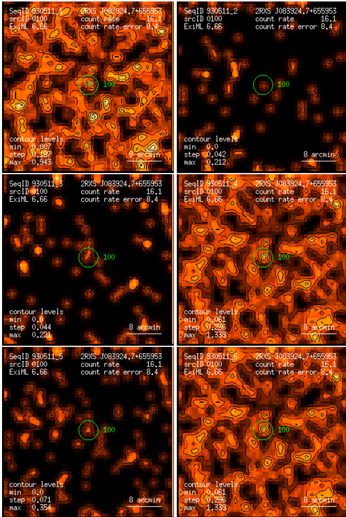
Figure 100: RASS 930511: detection 0100: band rate images, Gaussian filter: (1) PSPC channels 11 – 41, (2) 52 – 90, (3) 91 – 201, (4) 11 – 235, (5) 52 – 201, (6) 11 – 201. Broad band rates in counts/ks. Band rate contour levels in counts/ks/arcmin 2 .
