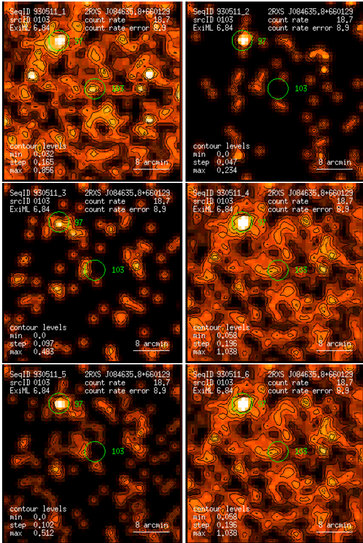
Figure 103: RASS 930511: detection 0103: band rate images, Gaussian filter: (1) PSPC channels 11 – 41, (2) 52 – 90, (3) 91 – 201, (4) 11 – 235, (5) 52 – 201, (6) 11 – 201. Broad band rates in counts/ks. Band rate contour levels in counts/ks/arcmin 2 .
