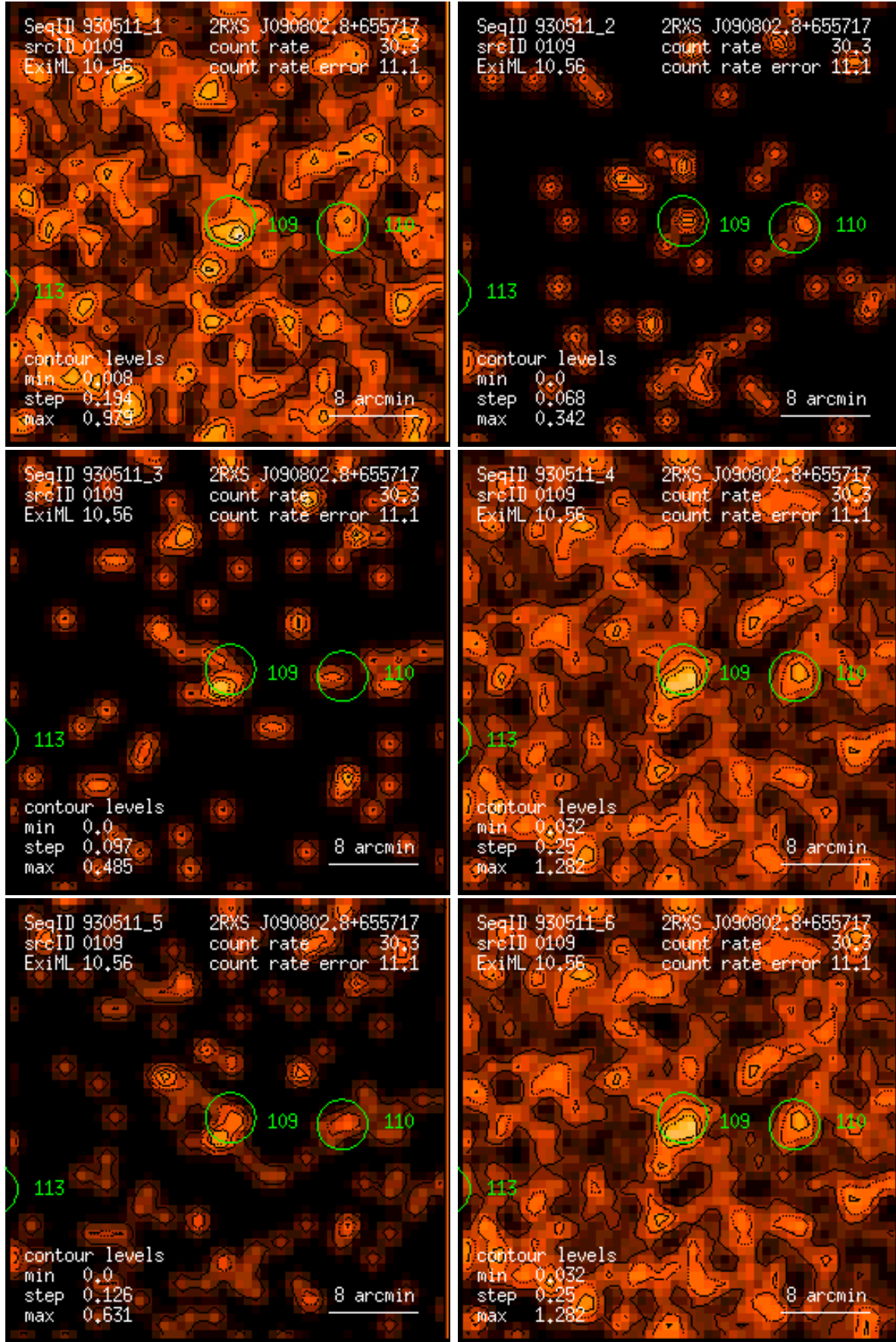
Figure 109: RASS 930511: detection 0109: band rate images, Gaussian filter: (1) PSPC channels 11 – 41, (2) 52 – 90, (3) 91 – 201, (4) 11 – 235, (5) 52 – 201, (6) 11 – 201. Broad band rates in counts/ks. Band rate contour levels in counts/ks/arcmin 2 .
