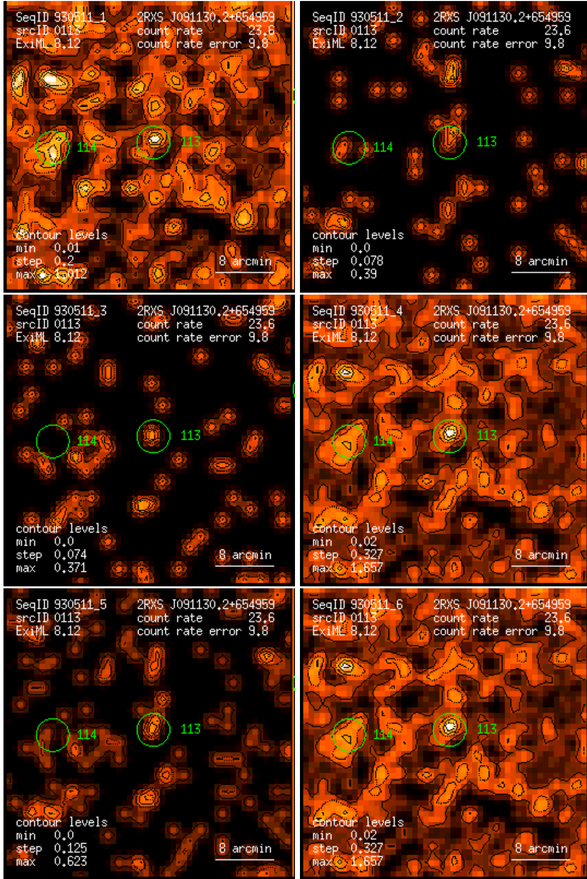
Figure 113: RASS 930511: detection 0113: band rate images, Gaussian filter: (1) PSPC channels 11 – 41, (2) 52 – 90, (3) 91 – 201, (4) 11 – 235, (5) 52 – 201, (6) 11 – 201. Broad band rates in counts/ks. Band rate contour levels in counts/ks/arcmin 2 .
