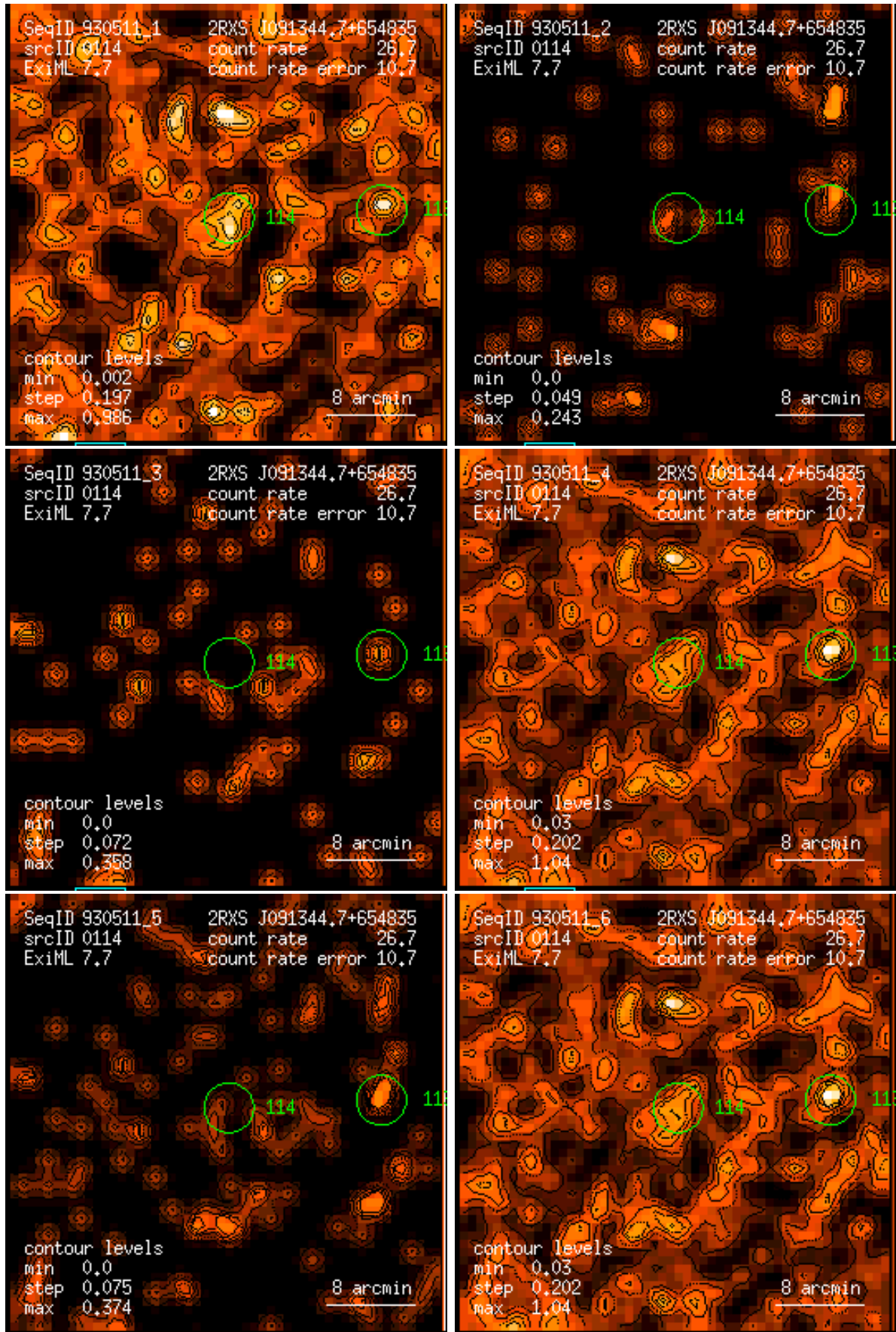
Figure 114: RASS 930511: detection 0114: band rate images, Gaussian filter: (1) PSPC channels 11 – 41, (2) 52 – 90, (3) 91 – 201, (4) 11 – 235, (5) 52 – 201, (6) 11 – 201. Broad band rates in counts/ks. Band rate contour levels in counts/ks/arcmin 2 .
