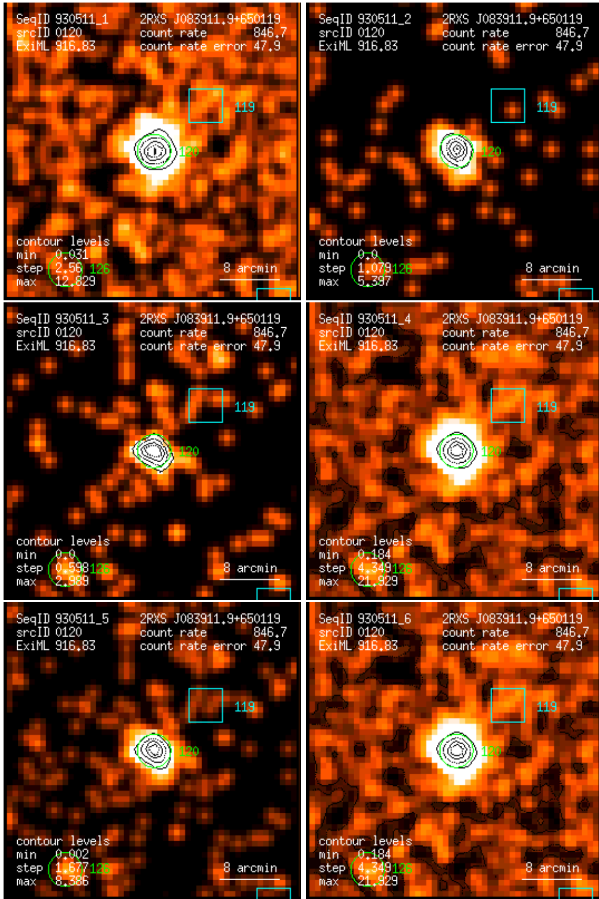
Figure 120: RASS 930511: detection 0120: band rate images, Gaussian filter: (1) PSPC channels 11 – 41, (2) 52 – 90, (3) 91 – 201, (4) 11 – 235, (5) 52 – 201, (6) 11 – 201. Broad band rates in counts/ks. Band rate contour levels in counts/ks/arcmin 2 .
