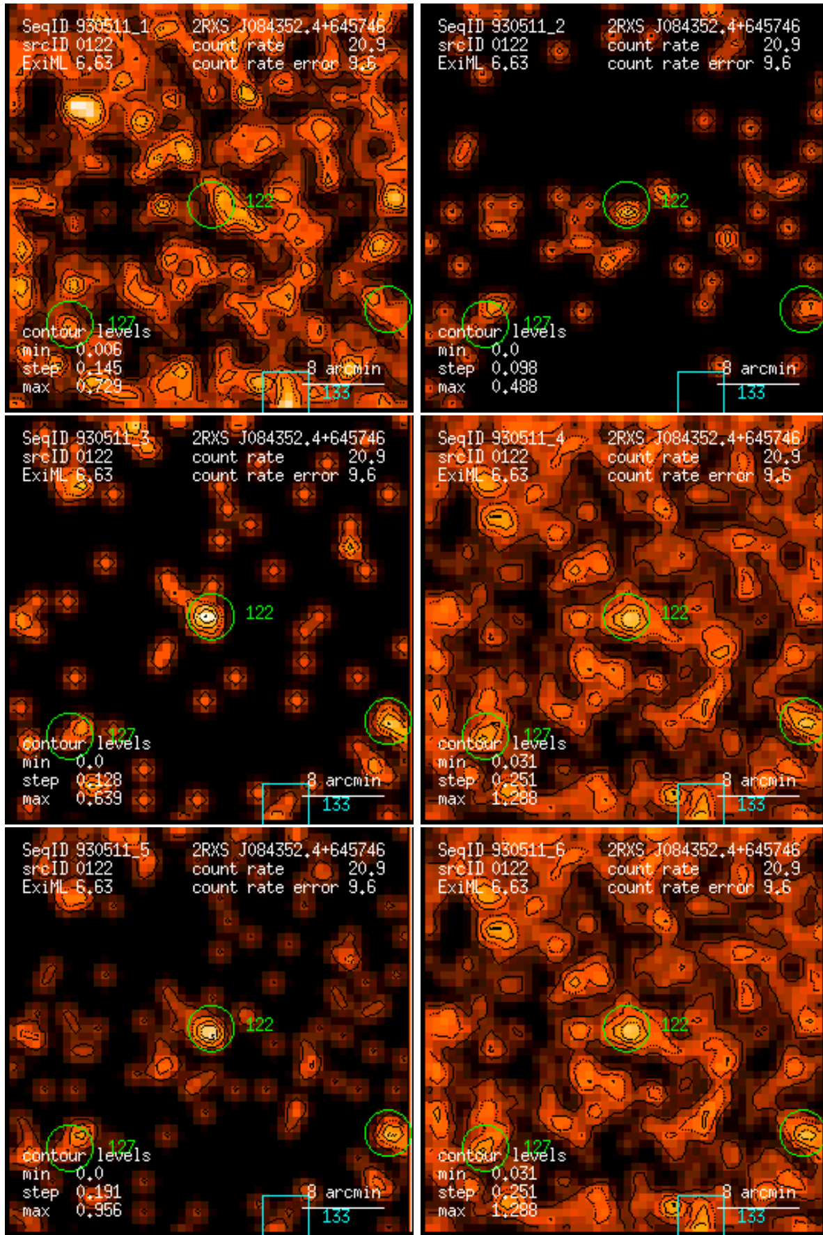
Figure 122: RASS 930511: detection 0122: band rate images, Gaussian filter: (1) PSPC channels 11 – 41, (2) 52 – 90, (3) 91 – 201, (4) 11 – 235, (5) 52 – 201, (6) 11 – 201. Broad band rates in counts/ks. Band rate contour levels in counts/ks/arcmin 2 .
