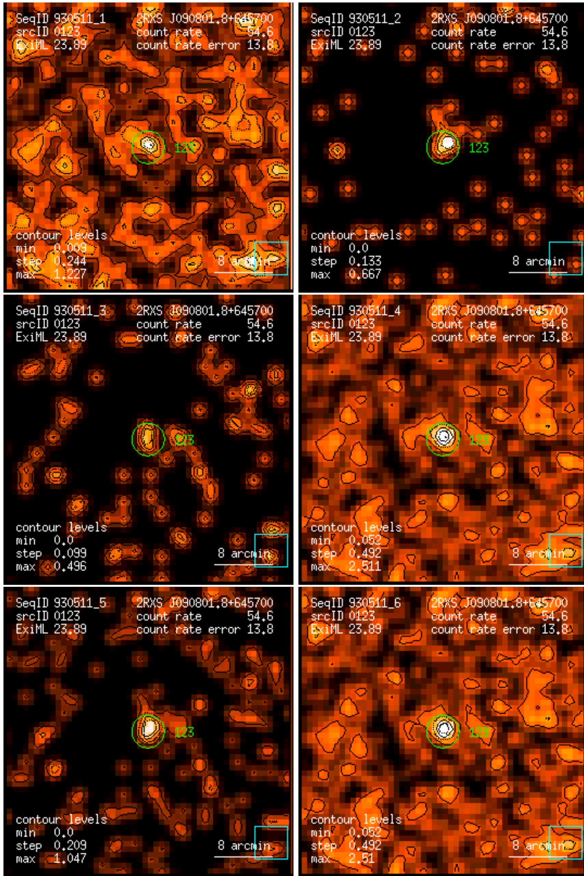
Figure 123: RASS 930511: detection 0123: band rate images, Gaussian filter: (1) PSPC channels 11 – 41, (2) 52 – 90, (3) 91 – 201, (4) 11 – 235, (5) 52 – 201, (6) 11 – 201. Broad band rates in counts/ks. Band rate contour levels in counts/ks/arcmin 2 .
