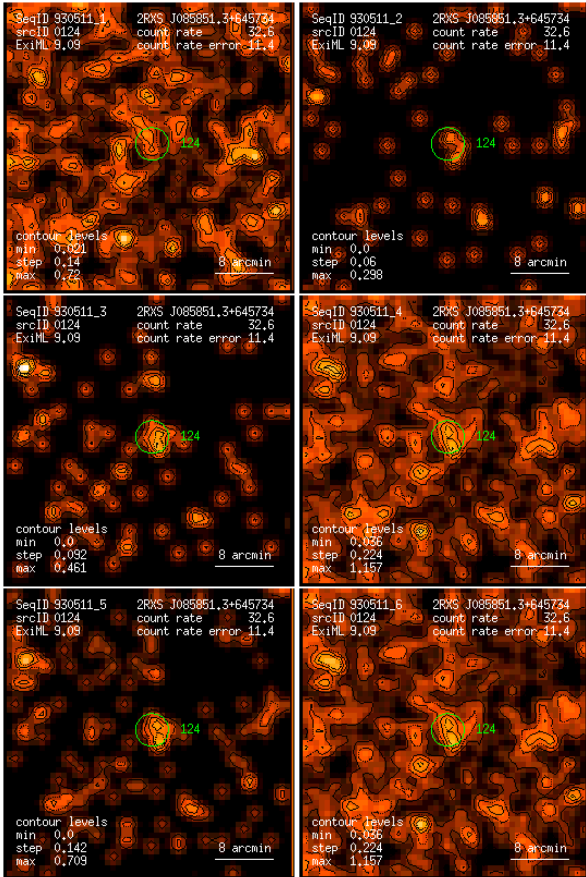
Figure 124: RASS 930511: detection 0124: band rate images, Gaussian filter: (1) PSPC channels 11 – 41, (2) 52 – 90, (3) 91 – 201, (4) 11 – 235, (5) 52 – 201, (6) 11 – 201. Broad band rates in counts/ks. Band rate contour levels in counts/ks/arcmin 2 .
