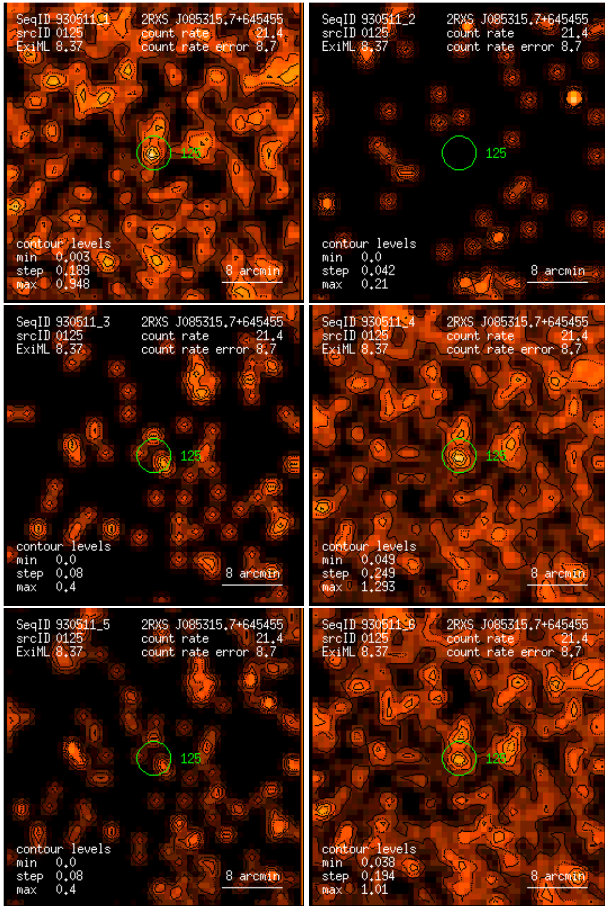
Figure 125: RASS 930511: detection 0125: band rate images, Gaussian filter: (1) PSPC channels 11 – 41, (2) 52 – 90, (3) 91 – 201, (4) 11 – 235, (5) 52 – 201, (6) 11 – 201. Broad band rates in counts/ks. Band rate contour levels in counts/ks/arcmin 2 .
