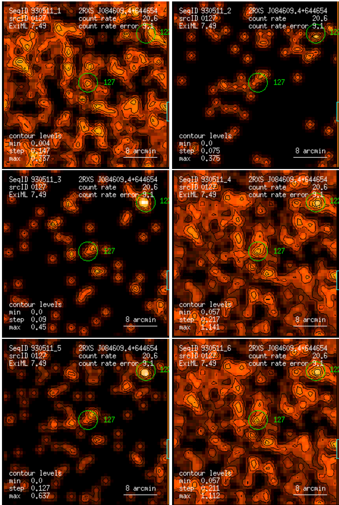
Figure 127: RASS 930511: detection 0127: band rate images, Gaussian filter: (1) PSPC channels 11 – 41, (2) 52 – 90, (3) 91 – 201, (4) 11 – 235, (5) 52 – 201, (6) 11 – 201. Broad band rates in counts/ks. Band rate contour levels in counts/ks/arcmin 2 .
