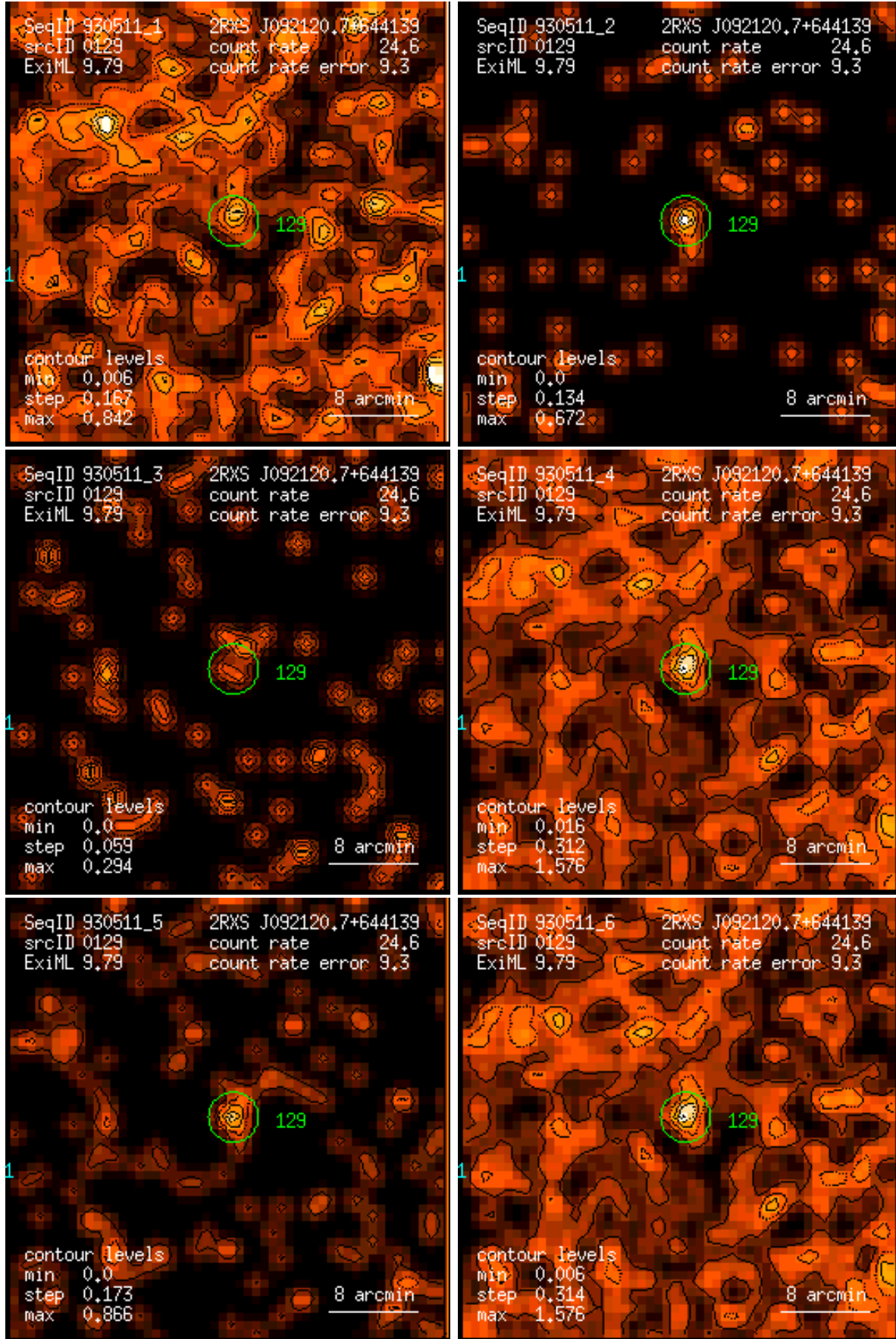
Figure 129: RASS 930511: detection 0129: band rate images, Gaussian filter: (1) PSPC channels 11 – 41, (2) 52 – 90, (3) 91 – 201, (4) 11 – 235, (5) 52 – 201, (6) 11 – 201. Broad band rates in counts/ks. Band rate contour levels in counts/ks/arcmin 2 .
