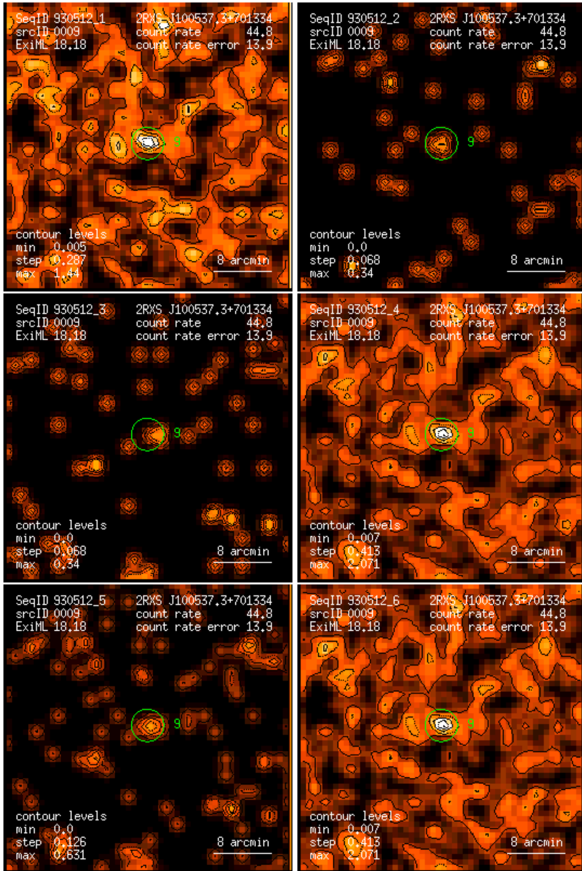
Figure 9: RASS 930512: detection 0009: band rate images, Gaussian filter: (1) PSPC channels 11 – 41, (2) 52 – 90, (3) 91 – 201, (4) 11 – 235, (5) 52 – 201, (6) 11 – 201. Broad band rates in counts/ks. Band rate contour levels in counts/ks/arcmin 2 .
