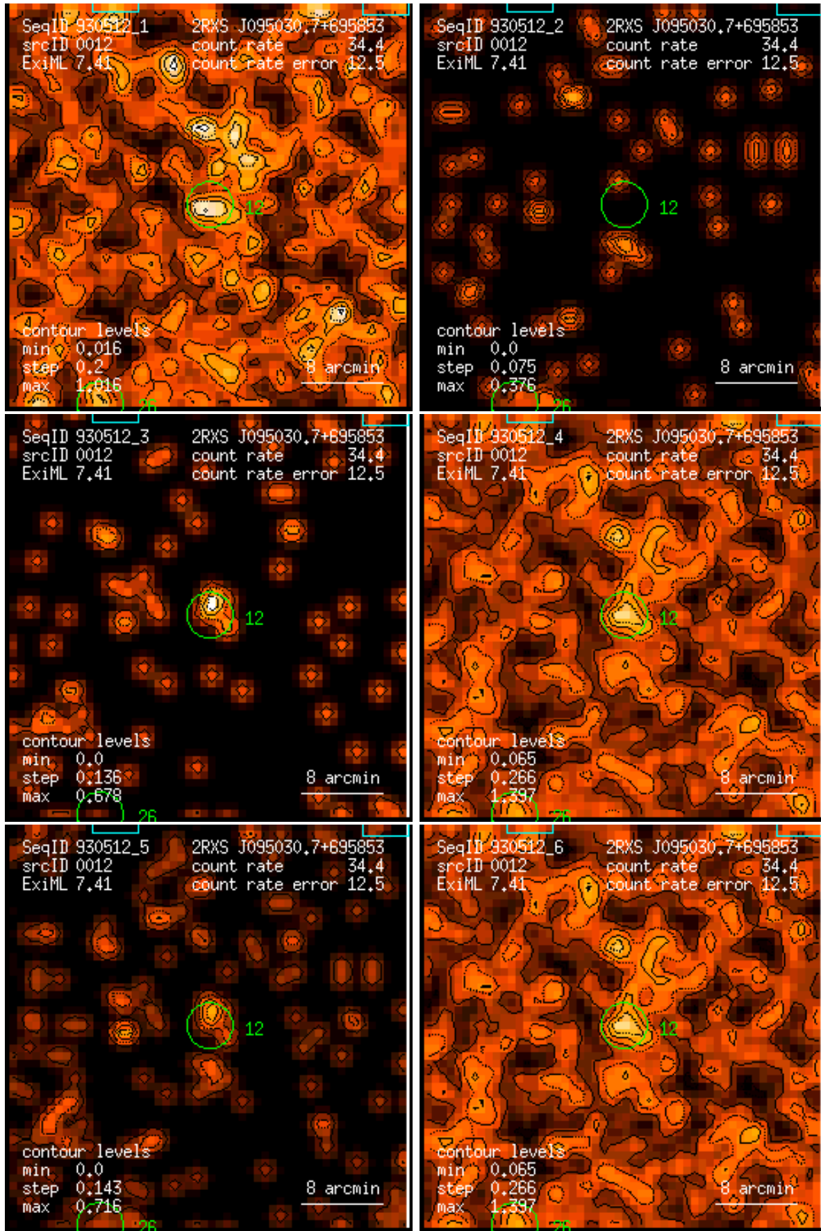
Figure 12: RASS 930512: detection 0012: band rate images, Gaussian filter: (1) PSPC channels 11 – 41, (2) 52 – 90, (3) 91 – 201, (4) 11 – 235, (5) 52 – 201, (6) 11 – 201. Broad band rates in counts/ks. Band rate contour levels in counts/ks/arcmin 2 .
