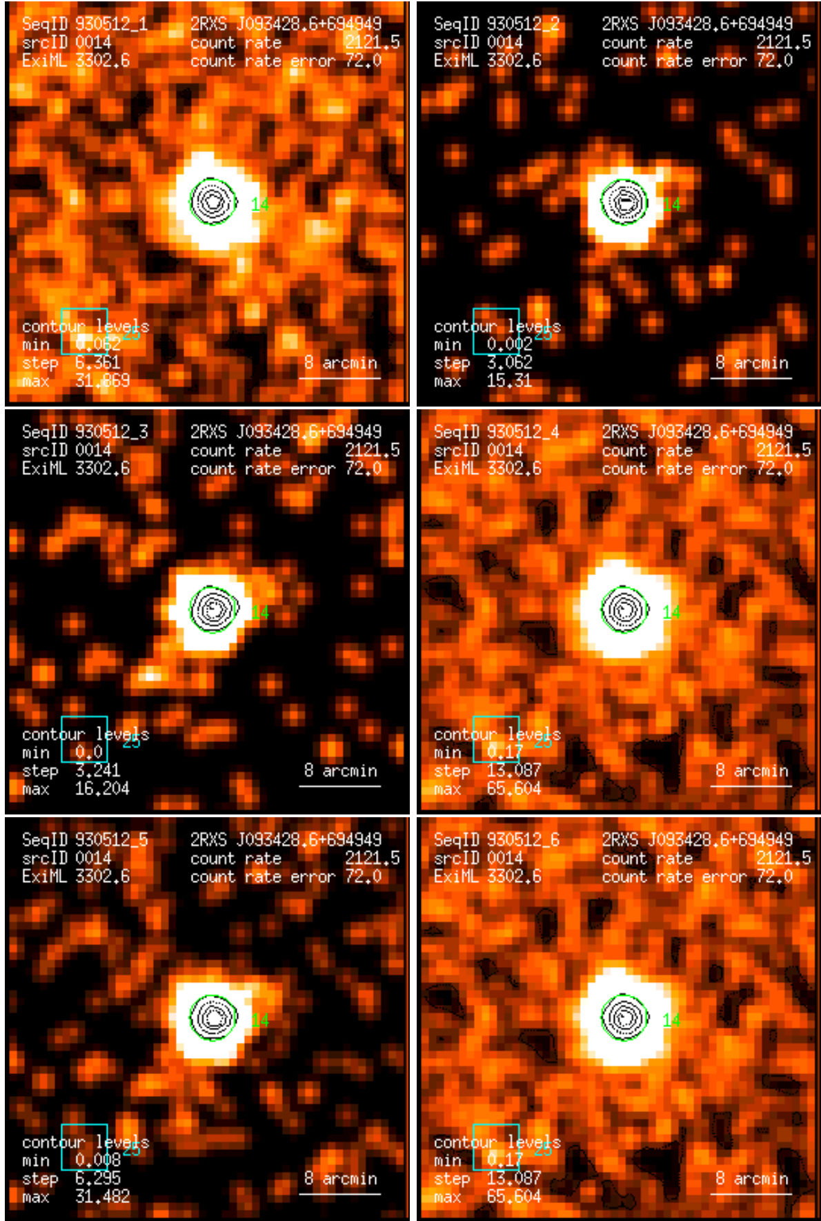
Figure 14: RASS 930512: detection 0014: band rate images, Gaussian filter: (1) PSPC channels 11 – 41, (2) 52 – 90, (3) 91 – 201, (4) 11 – 235, (5) 52 – 201, (6) 11 – 201. Broad band rates in counts/ks. Band rate contour levels in counts/ks/arcmin 2 .
