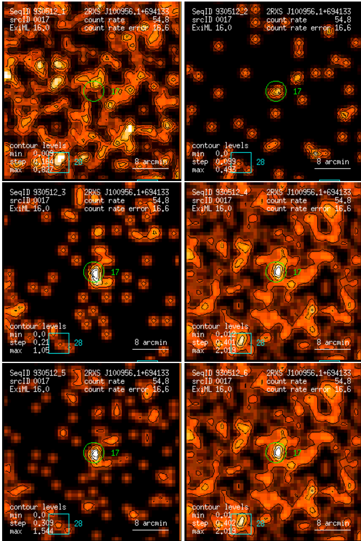
Figure 17: RASS 930512: detection 0017: band rate images, Gaussian filter: (1) PSPC channels 11 – 41, (2) 52 – 90, (3) 91 – 201, (4) 11 – 235, (5) 52 – 201, (6) 11 – 201. Broad band rates in counts/ks. Band rate contour levels in counts/ks/arcmin 2 .
