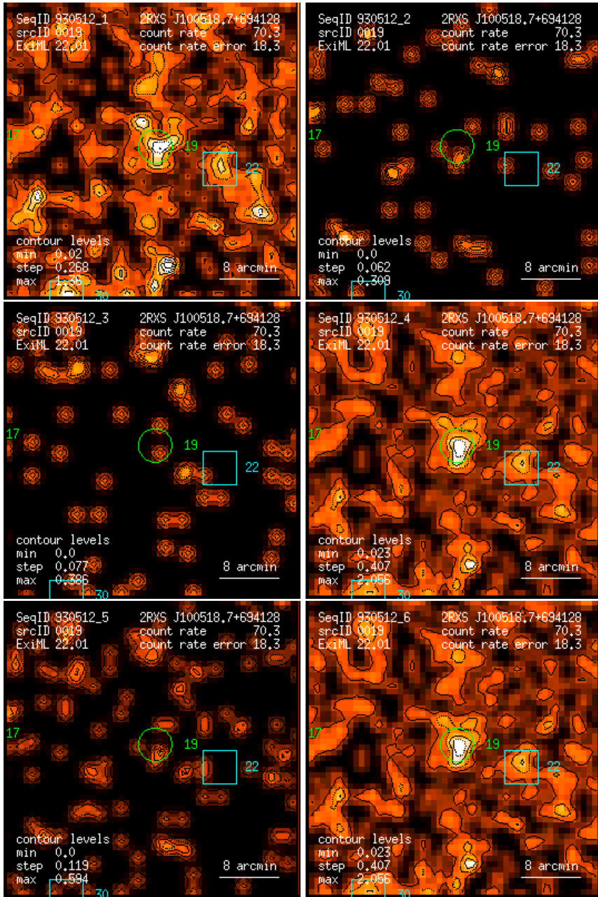
Figure 19: RASS 930512: detection 0019: band rate images, Gaussian filter: (1) PSPC channels 11 – 41, (2) 52 – 90, (3) 91 – 201, (4) 11 – 235, (5) 52 – 201, (6) 11 – 201. Broad band rates in counts/ks. Band rate contour levels in counts/ks/arcmin 2 .
