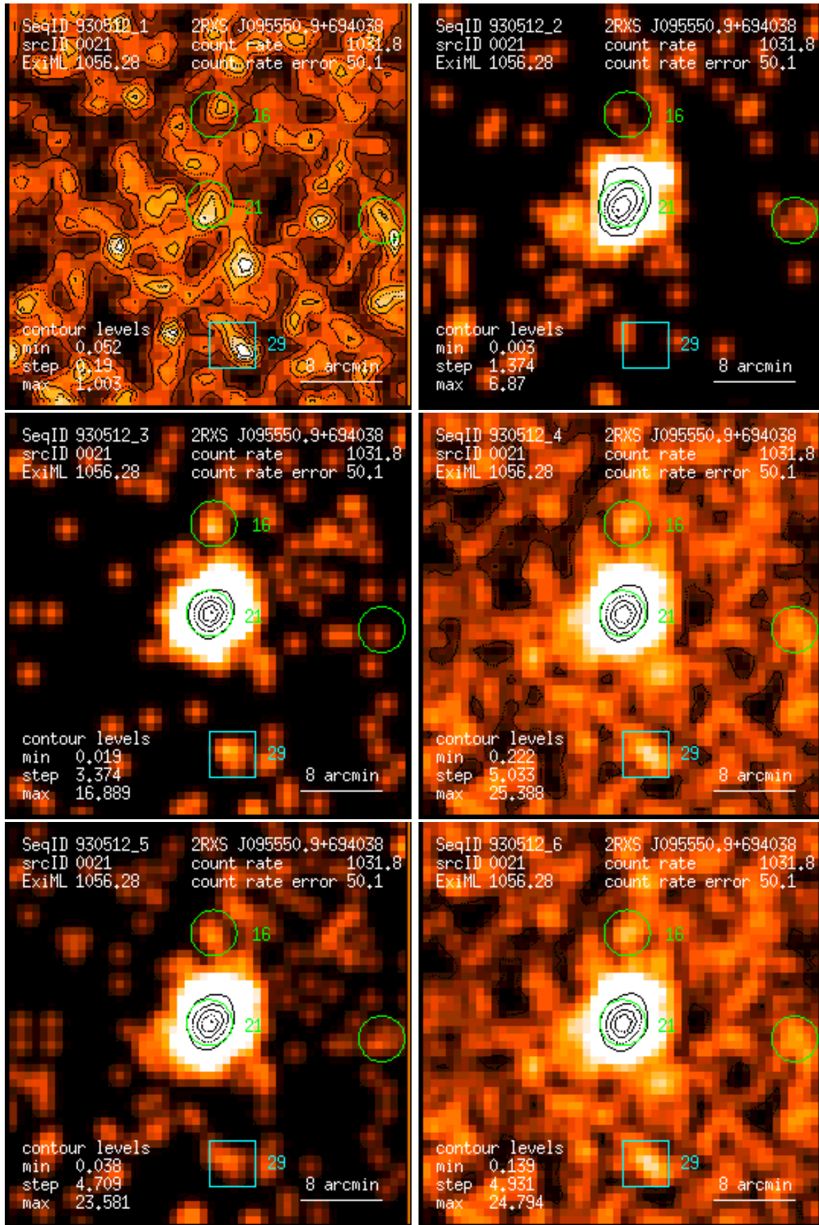
Figure 21: RASS 930512: detection 0021: band rate images, Gaussian filter: (1) PSPC channels 11 – 41, (2) 52 – 90, (3) 91 – 201, (4) 11 – 235, (5) 52 – 201, (6) 11 – 201. Broad band rates in counts/ks. Band rate contour levels in counts/ks/arcmin 2 .
