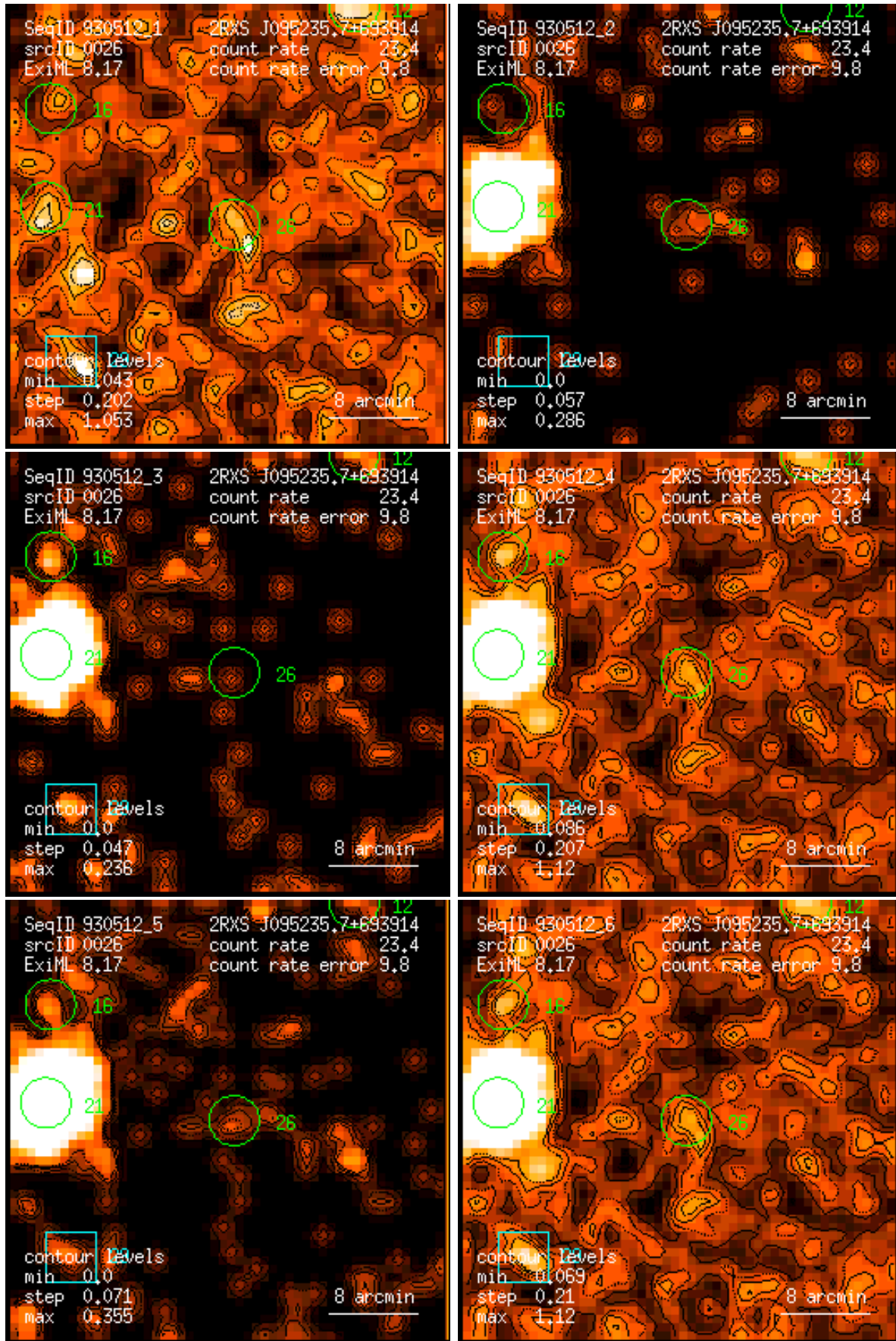
Figure 26: RASS 930512: detection 0026: band rate images, Gaussian filter: (1) PSPC channels 11 – 41, (2) 52 – 90, (3) 91 – 201, (4) 11 – 235, (5) 52 – 201, (6) 11 – 201. Broad band rates in counts/ks. Band rate contour levels in counts/ks/arcmin 2 .
