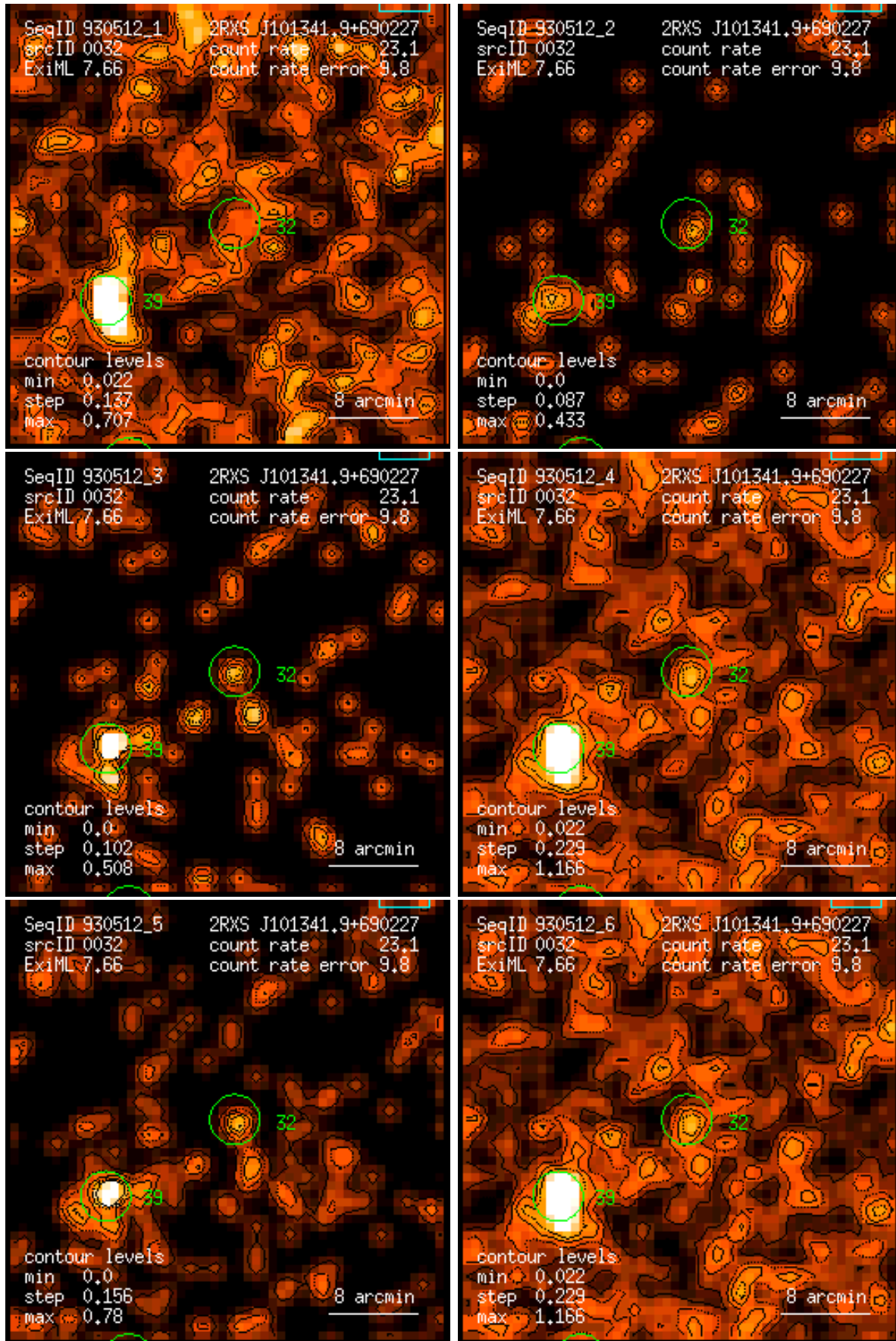
Figure 32: RASS 930512: detection 0032: band rate images, Gaussian filter: (1) PSPC channels 11 – 41, (2) 52 – 90, (3) 91 – 201, (4) 11 – 235, (5) 52 – 201, (6) 11 – 201. Broad band rates in counts/ks. Band rate contour levels in counts/ks/arcmin 2 .
