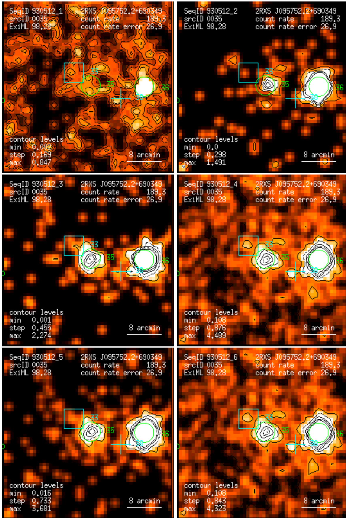
Figure 35: RASS 930512: detection 0035: band rate images, Gaussian filter: (1) PSPC channels 11 – 41, (2) 52 – 90, (3) 91 – 201, (4) 11 – 235, (5) 52 – 201, (6) 11 – 201. Broad band rates in counts/ks. Band rate contour levels in counts/ks/arcmin 2 .
