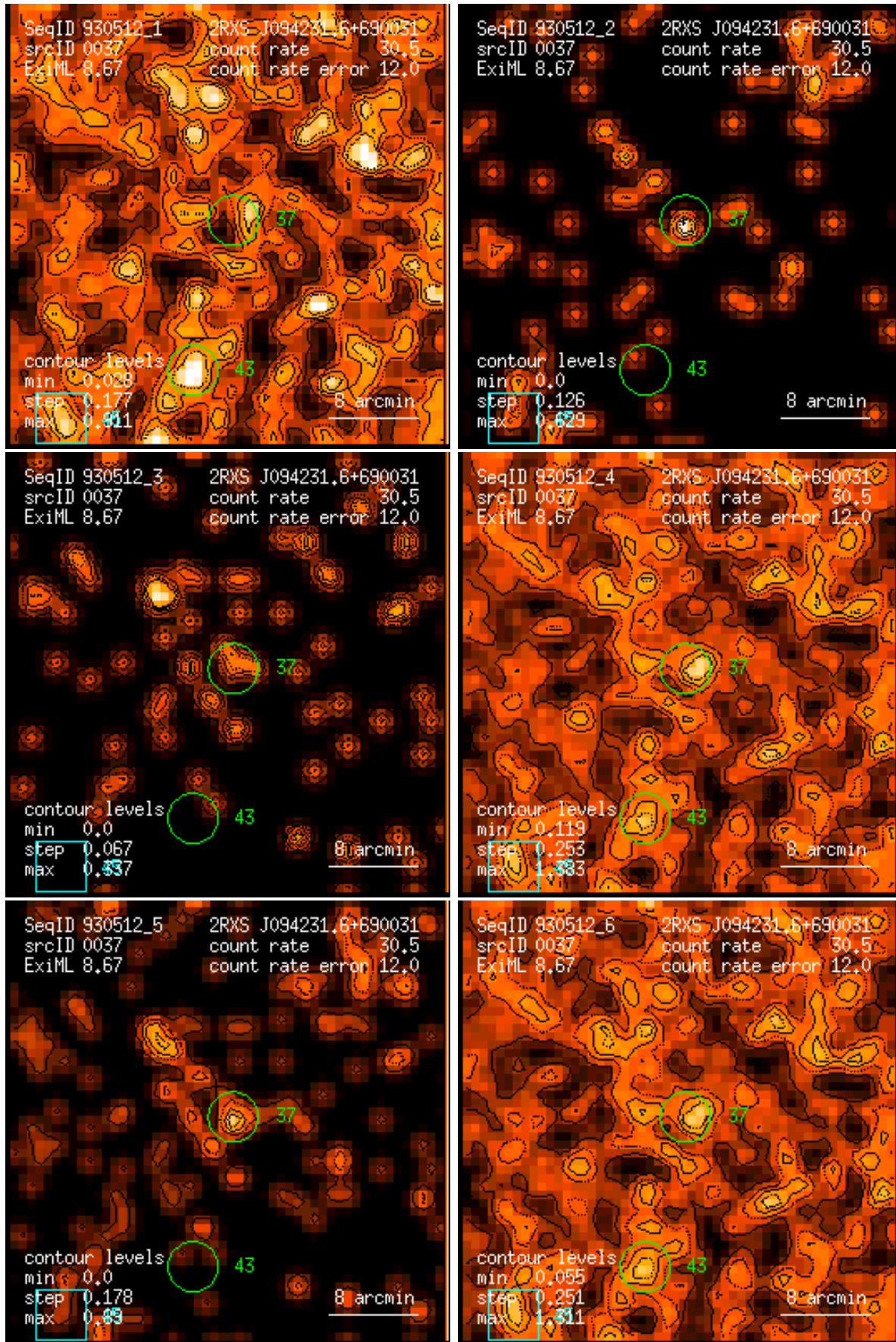
Figure 37: RASS 930512: detection 0037: band rate images, Gaussian filter: (1) PSPC channels 11 – 41, (2) 52 – 90, (3) 91 – 201, (4) 11 – 235, (5) 52 – 201, (6) 11 – 201. Broad band rates in counts/ks. Band rate contour levels in counts/ks/arcmin 2 .
