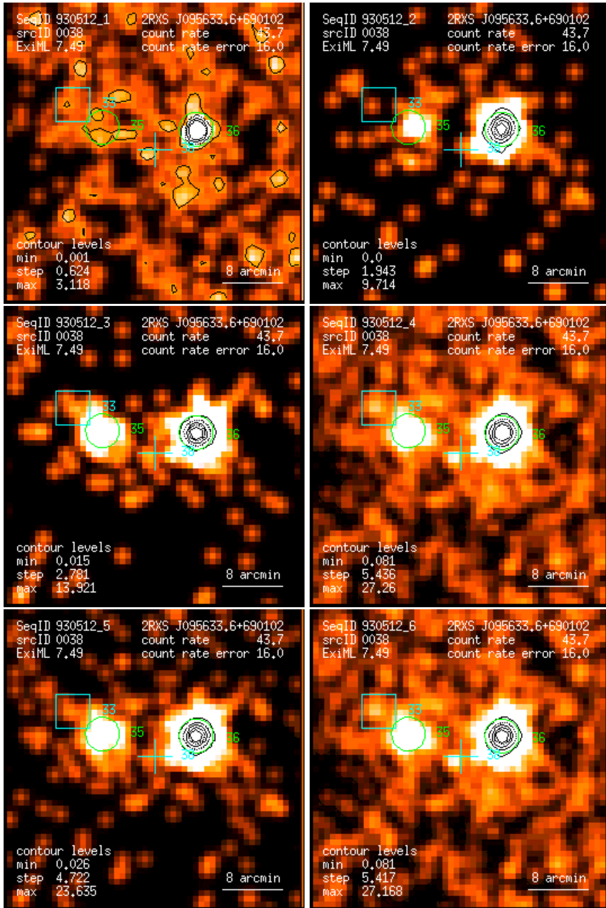
Figure 38: RASS 930512: detection 0038: band rate images, Gaussian filter: (1) PSPC channels 11 – 41, (2) 52 – 90, (3) 91 – 201, (4) 11 – 235, (5) 52 – 201, (6) 11 – 201. Broad band rates in counts/ks. Band rate contour levels in counts/ks/arcmin 2 .
