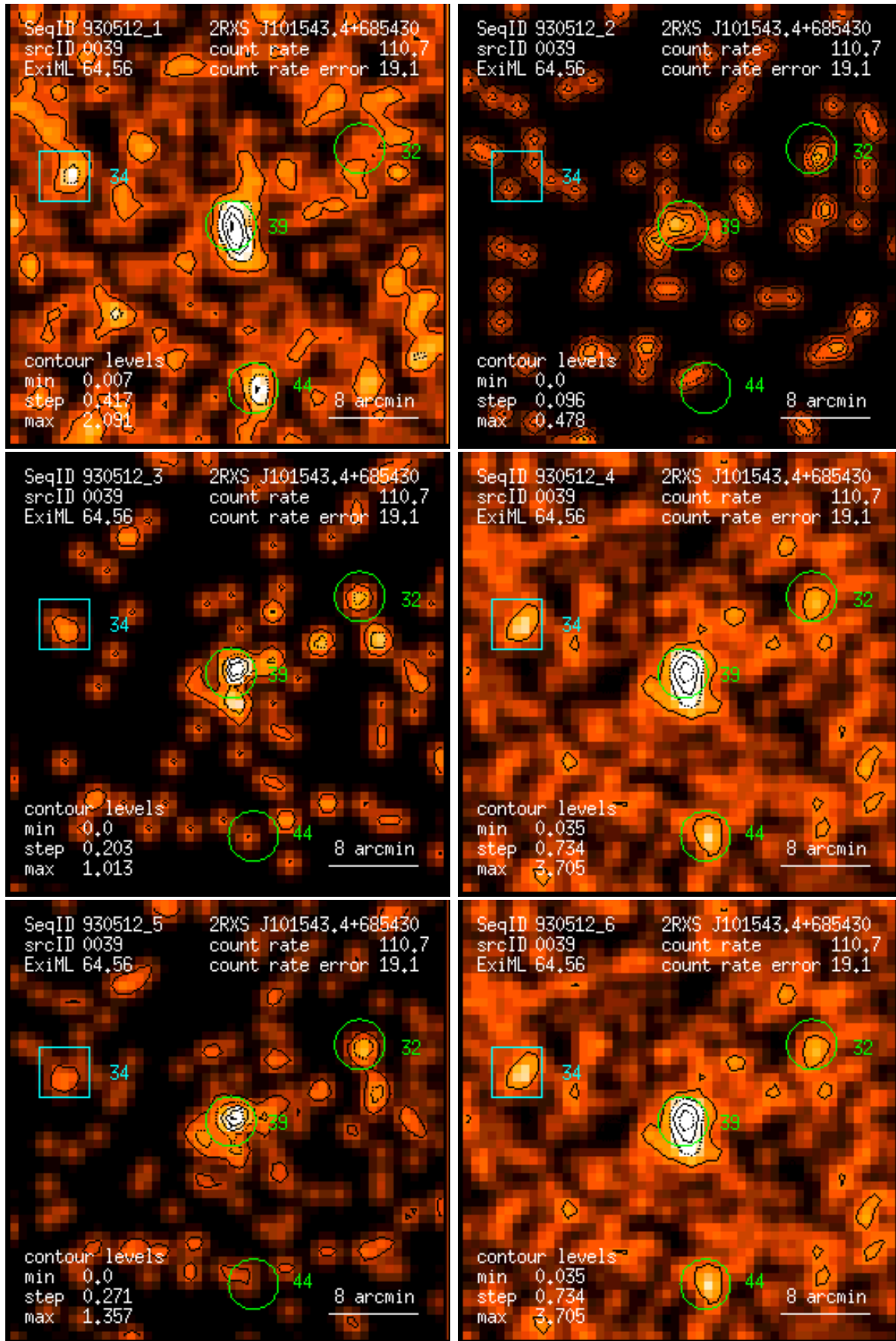
Figure 39: RASS 930512: detection 0039: band rate images, Gaussian filter: (1) PSPC channels 11 – 41, (2) 52 – 90, (3) 91 – 201, (4) 11 – 235, (5) 52 – 201, (6) 11 – 201. Broad band rates in counts/ks. Band rate contour levels in counts/ks/arcmin 2 .
