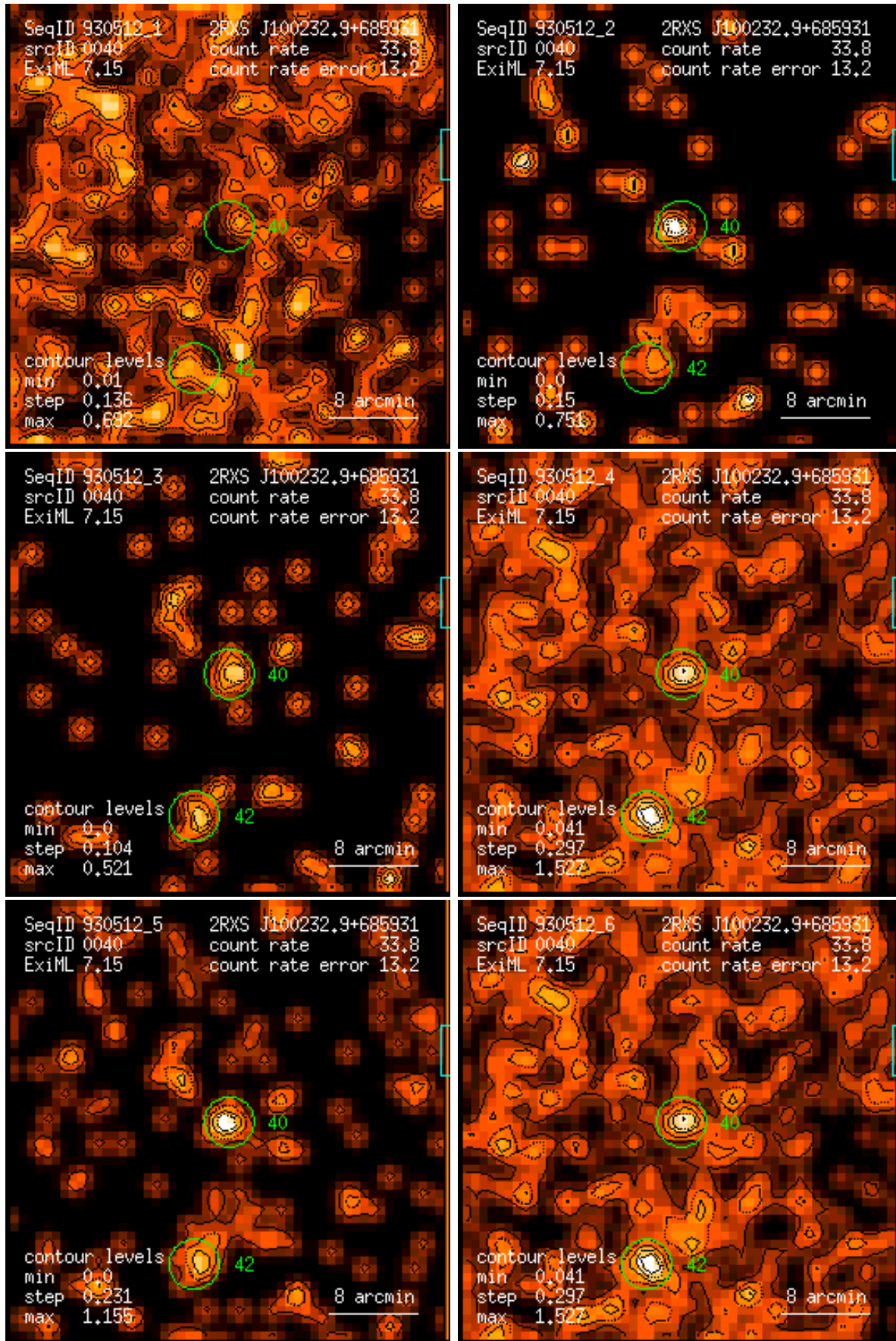
Figure 40: RASS 930512: detection 0040: band rate images, Gaussian filter: (1) PSPC channels 11 – 41, (2) 52 – 90, (3) 91 – 201, (4) 11 – 235, (5) 52 – 201, (6) 11 – 201. Broad band rates in counts/ks. Band rate contour levels in counts/ks/arcmin 2 .
