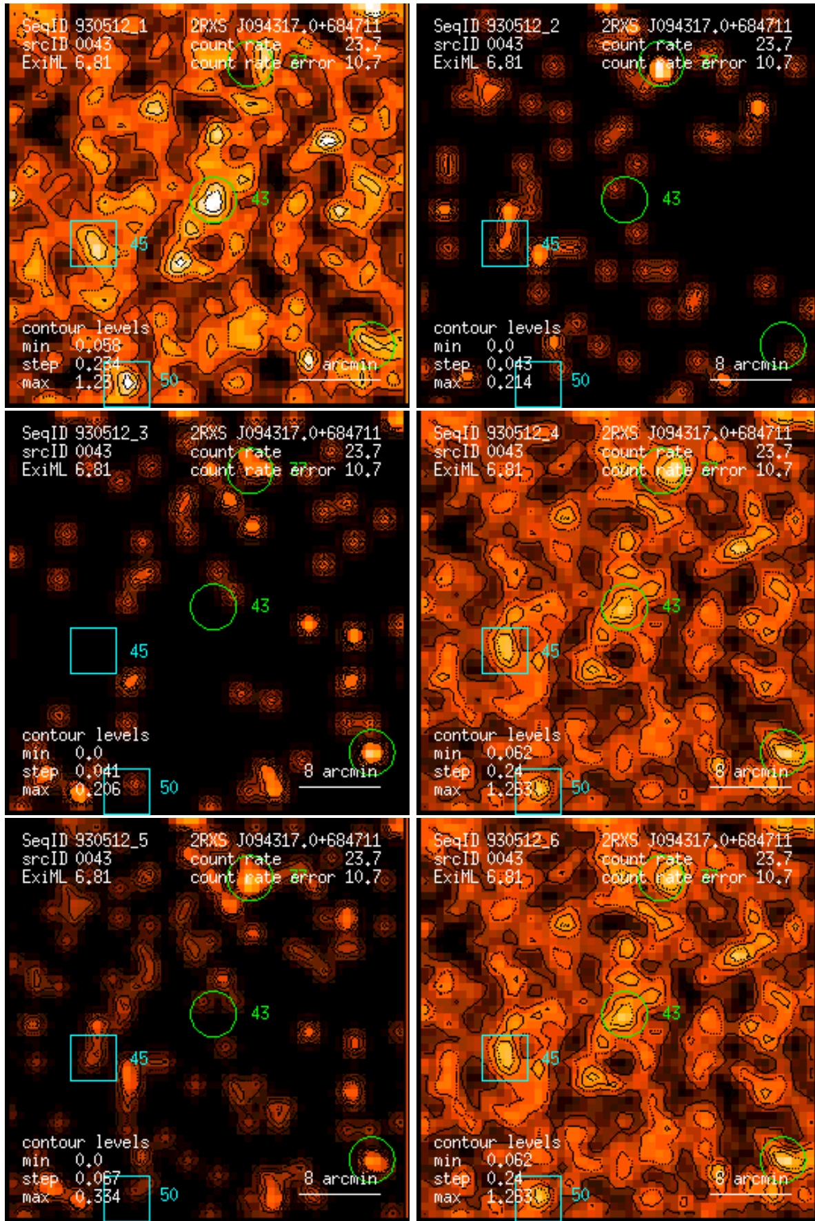
Figure 43: RASS 930512: detection 0043: band rate images, Gaussian filter: (1) PSPC channels 11 – 41, (2) 52 – 90, (3) 91 – 201, (4) 11 – 235, (5) 52 – 201, (6) 11 – 201. Broad band rates in counts/ks. Band rate contour levels in counts/ks/arcmin 2 .
