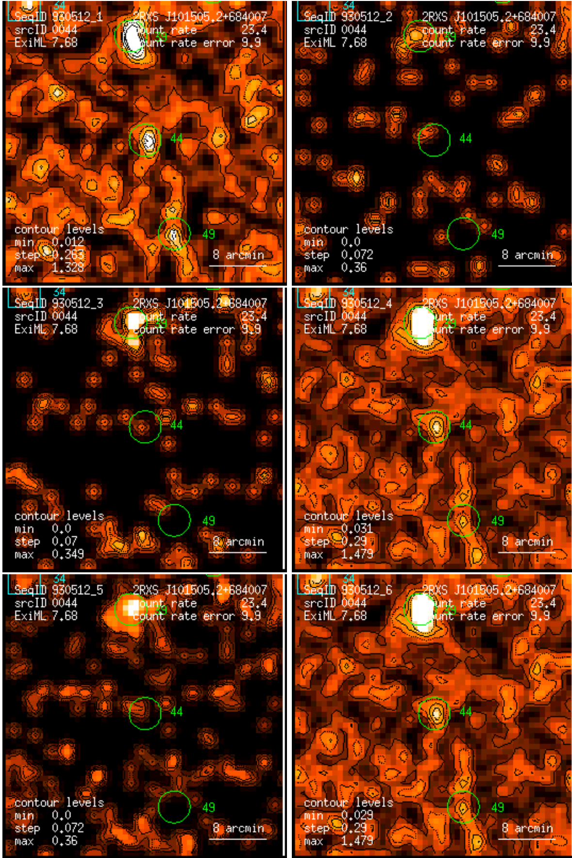
Figure 44: RASS 930512: detection 0044: band rate images, Gaussian filter: (1) PSPC channels 11 – 41, (2) 52 – 90, (3) 91 – 201, (4) 11 – 235, (5) 52 – 201, (6) 11 – 201. Broad band rates in counts/ks. Band rate contour levels in counts/ks/arcmin 2 .
