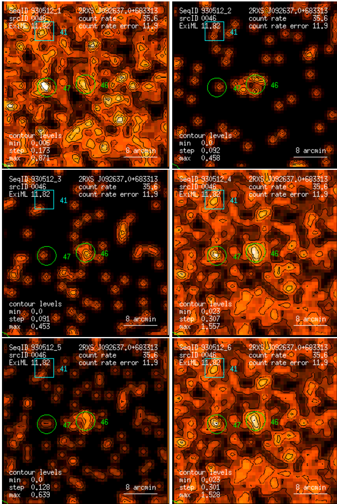
Figure 46: RASS 930512: detection 0046: band rate images, Gaussian filter: (1) PSPC channels 11 – 41, (2) 52 – 90, (3) 91 – 201, (4) 11 – 235, (5) 52 – 201, (6) 11 – 201. Broad band rates in counts/ks. Band rate contour levels in counts/ks/arcmin 2 .
