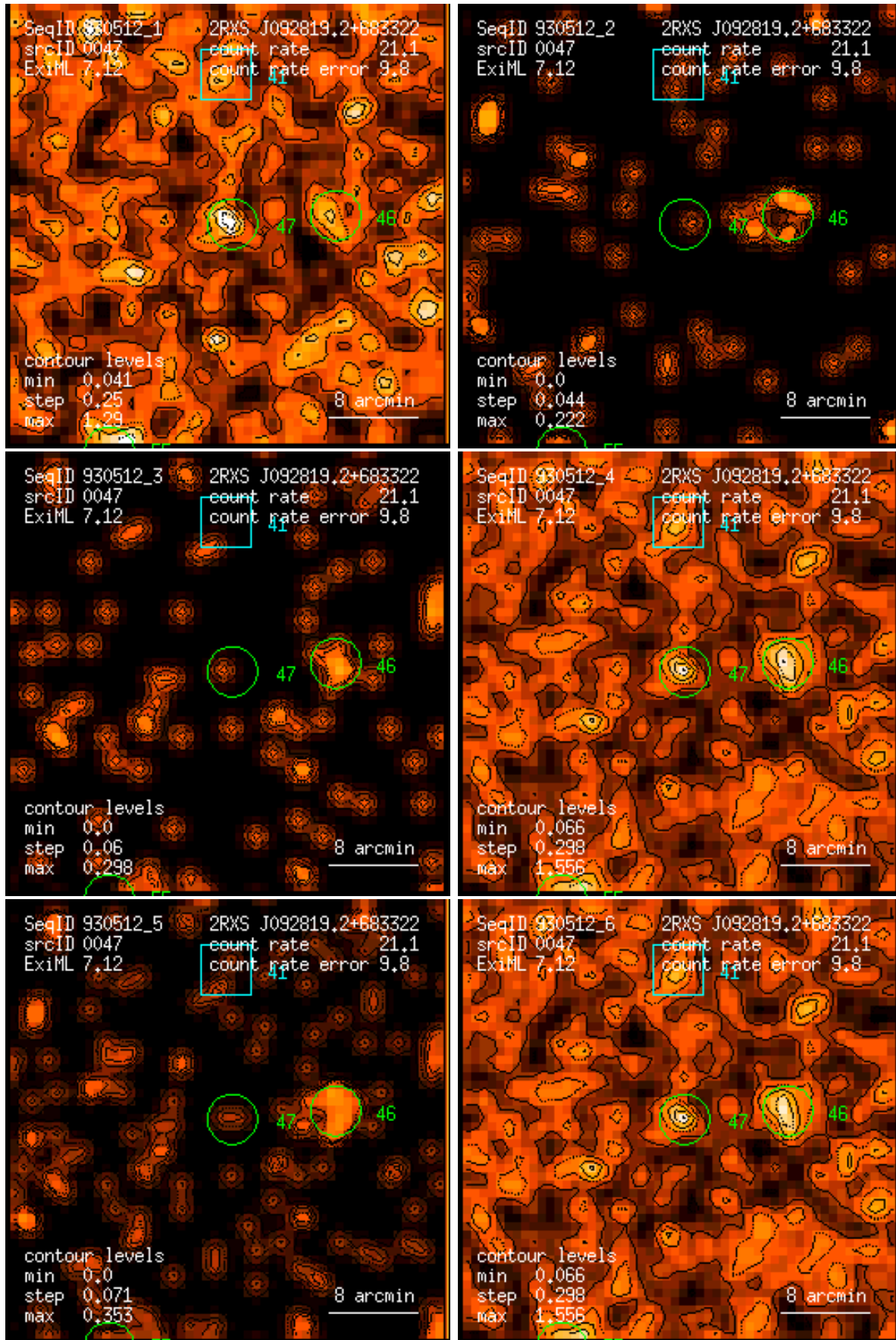
Figure 47: RASS 930512: detection 0047: band rate images, Gaussian filter: (1) PSPC channels 11 – 41, (2) 52 – 90, (3) 91 – 201, (4) 11 – 235, (5) 52 – 201, (6) 11 – 201. Broad band rates in counts/ks. Band rate contour levels in counts/ks/arcmin 2 .
