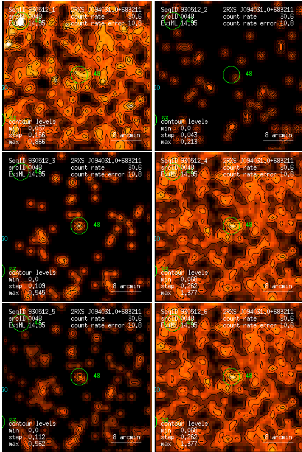
Figure 48: RASS 930512: detection 0048: band rate images, Gaussian filter: (1) PSPC channels 11 – 41, (2) 52 – 90, (3) 91 – 201, (4) 11 – 235, (5) 52 – 201, (6) 11 – 201. Broad band rates in counts/ks. Band rate contour levels in counts/ks/arcmin 2 .
