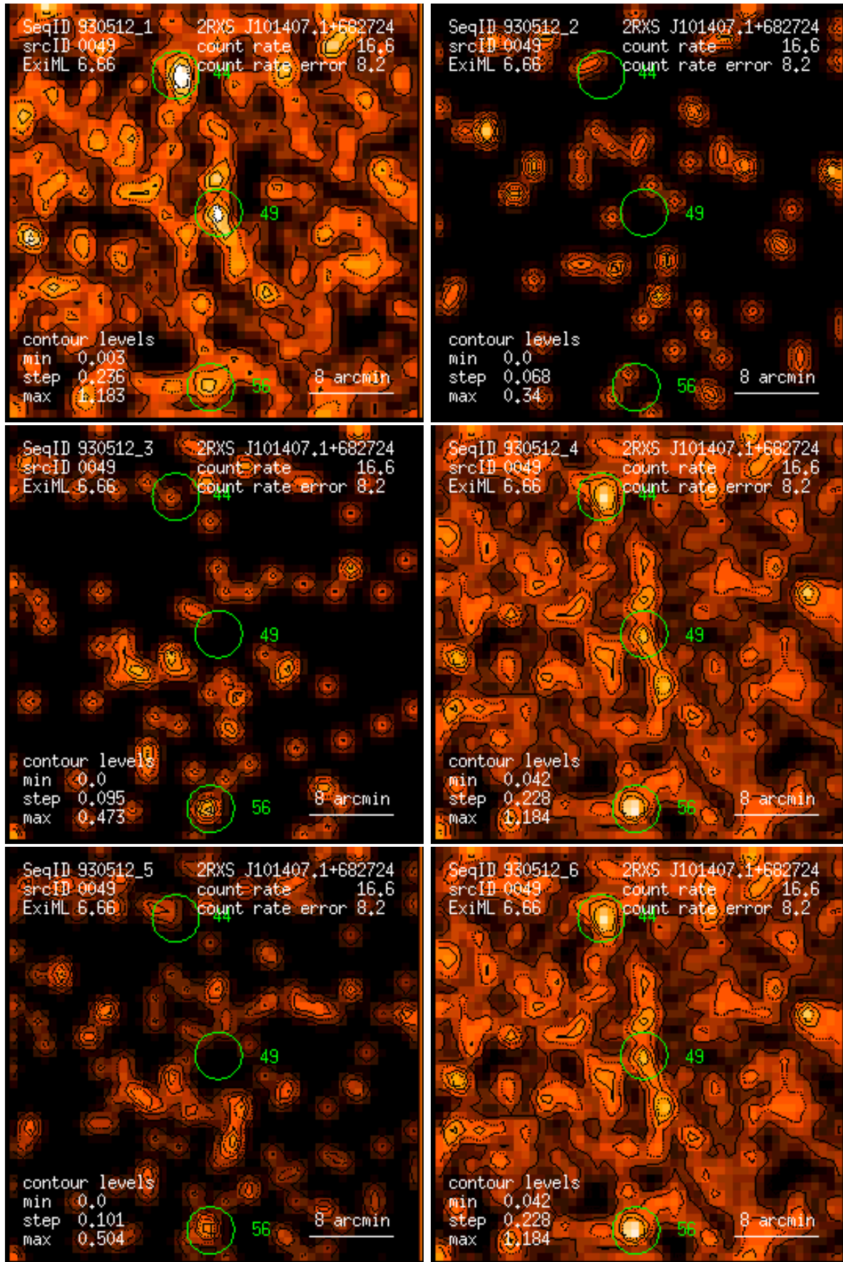
Figure 49: RASS 930512: detection 0049: band rate images, Gaussian filter: (1) PSPC channels 11 – 41, (2) 52 – 90, (3) 91 – 201, (4) 11 – 235, (5) 52 – 201, (6) 11 – 201. Broad band rates in counts/ks. Band rate contour levels in counts/ks/arcmin 2 .
