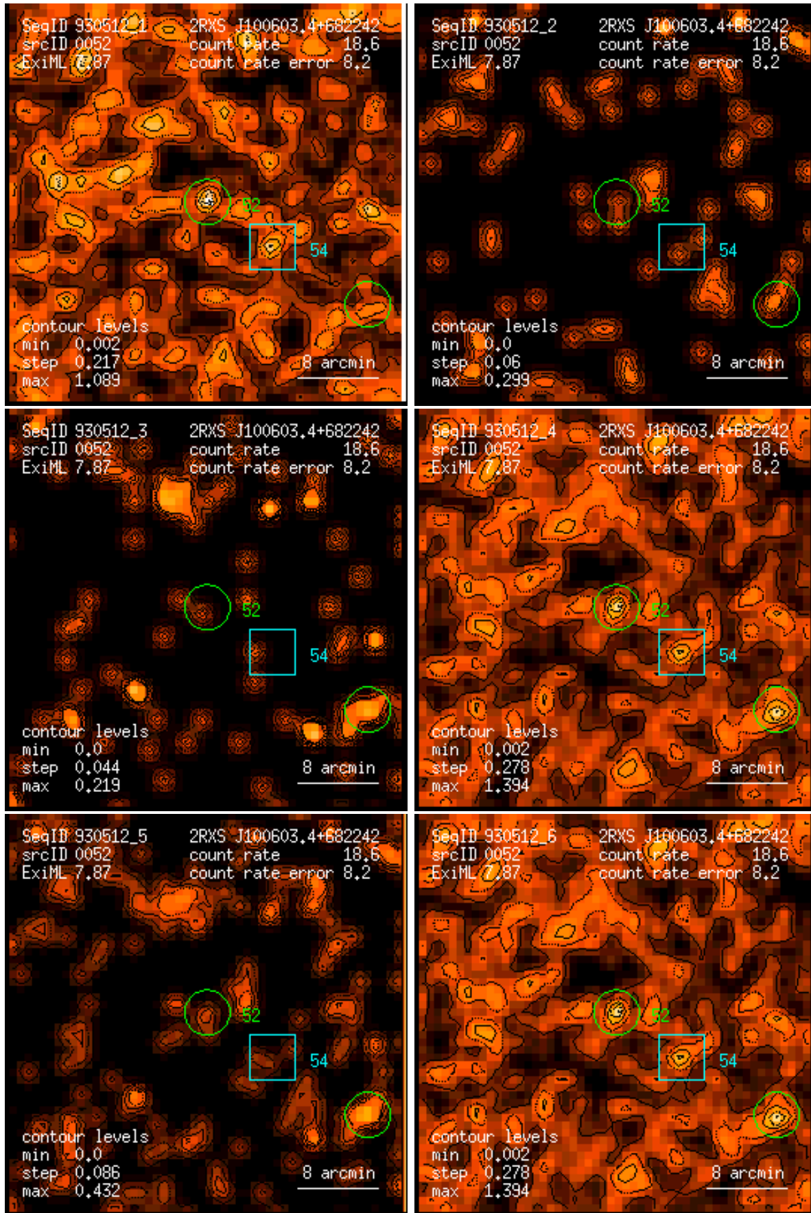
Figure 52: RASS 930512: detection 0052: band rate images, Gaussian filter: (1) PSPC channels 11 – 41, (2) 52 – 90, (3) 91 – 201, (4) 11 – 235, (5) 52 – 201, (6) 11 – 201. Broad band rates in counts/ks. Band rate contour levels in counts/ks/arcmin 2 .
