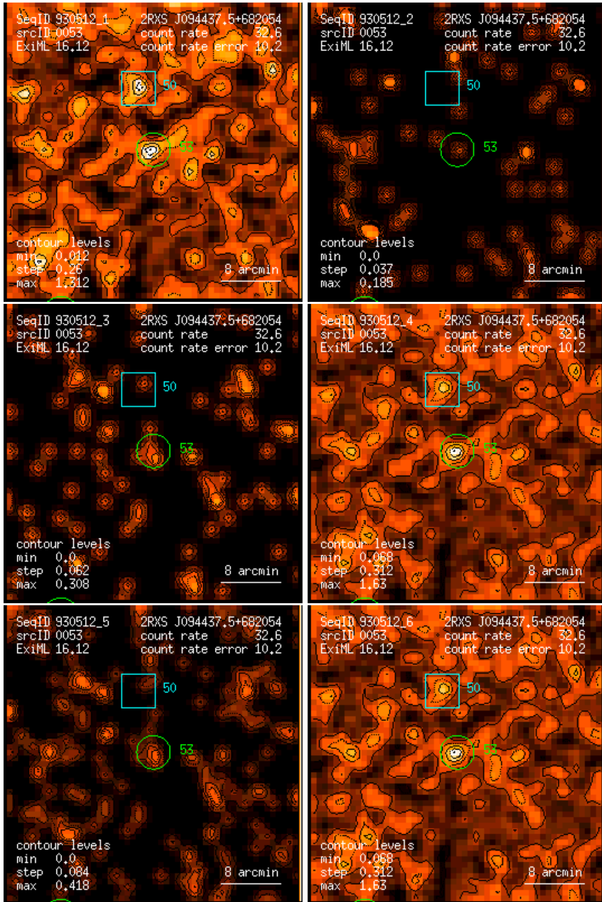
Figure 53: RASS 930512: detection 0053: band rate images, Gaussian filter: (1) PSPC channels 11 – 41, (2) 52 – 90, (3) 91 – 201, (4) 11 – 235, (5) 52 – 201, (6) 11 – 201. Broad band rates in counts/ks. Band rate contour levels in counts/ks/arcmin 2 .
