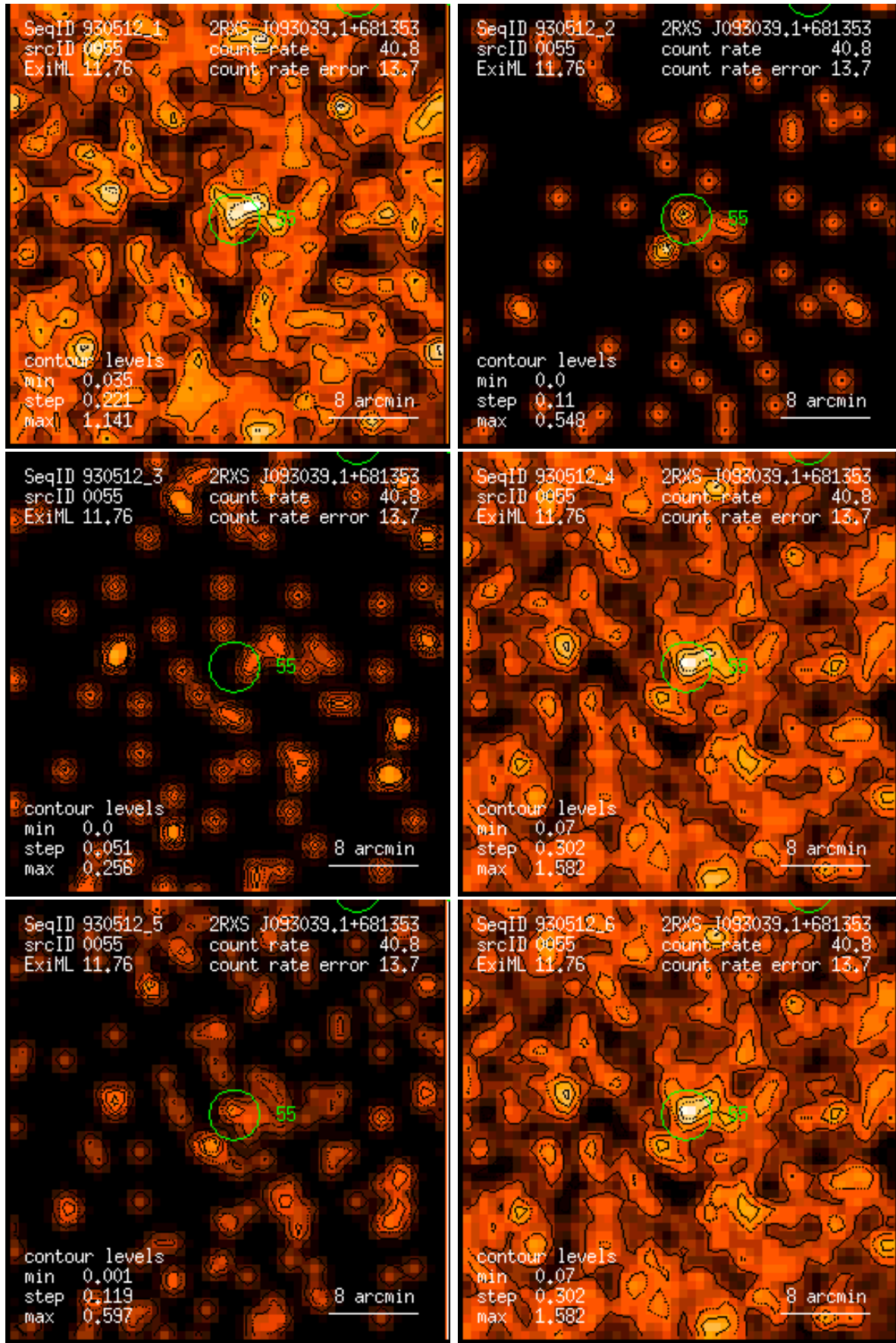
Figure 55: RASS 930512: detection 0055: band rate images, Gaussian filter: (1) PSPC channels 11 – 41, (2) 52 – 90, (3) 91 – 201, (4) 11 – 235, (5) 52 – 201, (6) 11 – 201. Broad band rates in counts/ks. Band rate contour levels in counts/ks/arcmin 2 .
