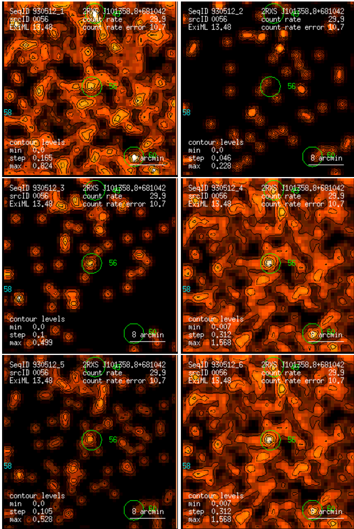
Figure 56: RASS 930512: detection 0056: band rate images, Gaussian filter: (1) PSPC channels 11 – 41, (2) 52 – 90, (3) 91 – 201, (4) 11 – 235, (5) 52 – 201, (6) 11 – 201. Broad band rates in counts/ks. Band rate contour levels in counts/ks/arcmin 2 .
