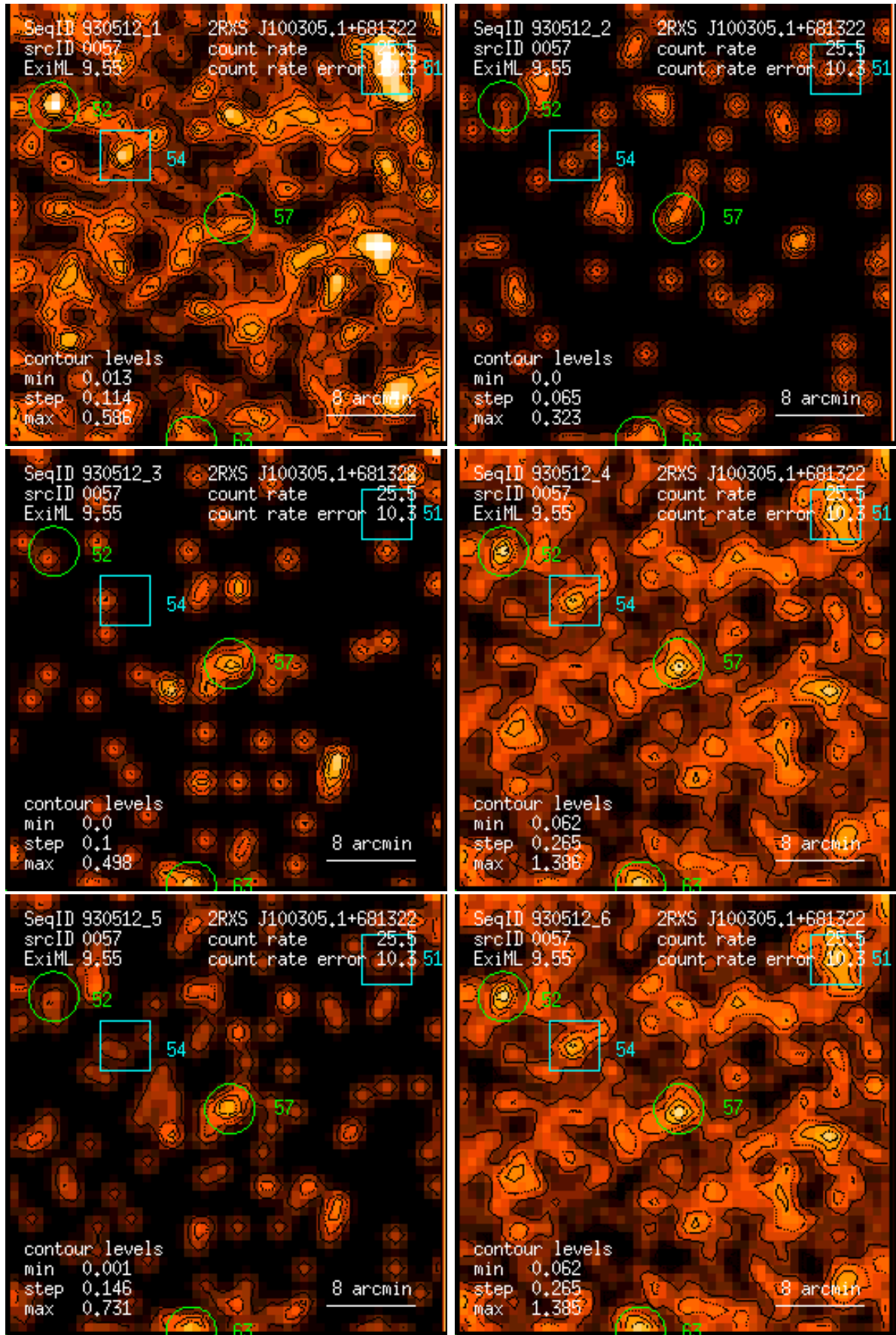
Figure 57: RASS 930512: detection 0057: band rate images, Gaussian filter: (1) PSPC channels 11 – 41, (2) 52 – 90, (3) 91 – 201, (4) 11 – 235, (5) 52 – 201, (6) 11 – 201. Broad band rates in counts/ks. Band rate contour levels in counts/ks/arcmin 2 .
