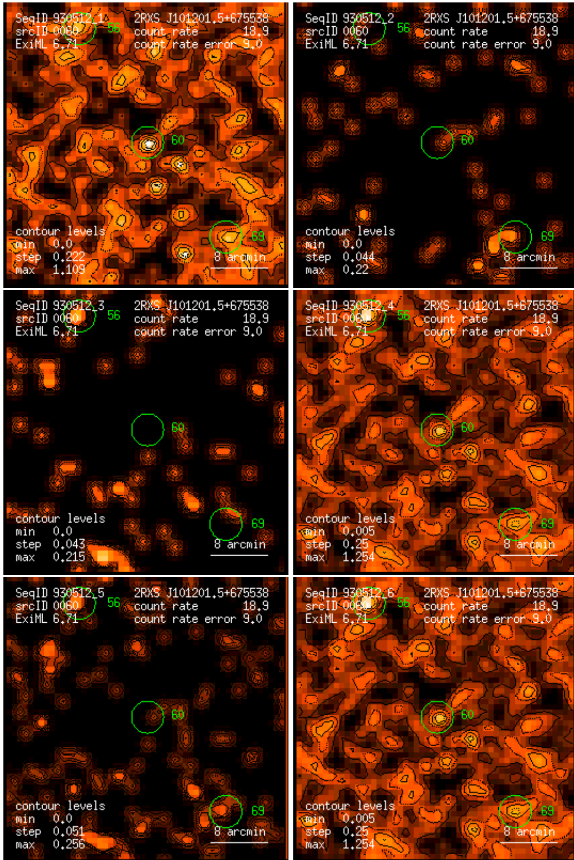
Figure 60: RASS 930512: detection 0060: band rate images, Gaussian filter: (1) PSPC channels 11 – 41, (2) 52 – 90, (3) 91 – 201, (4) 11 – 235, (5) 52 – 201, (6) 11 – 201. Broad band rates in counts/ks. Band rate contour levels in counts/ks/arcmin 2 .
