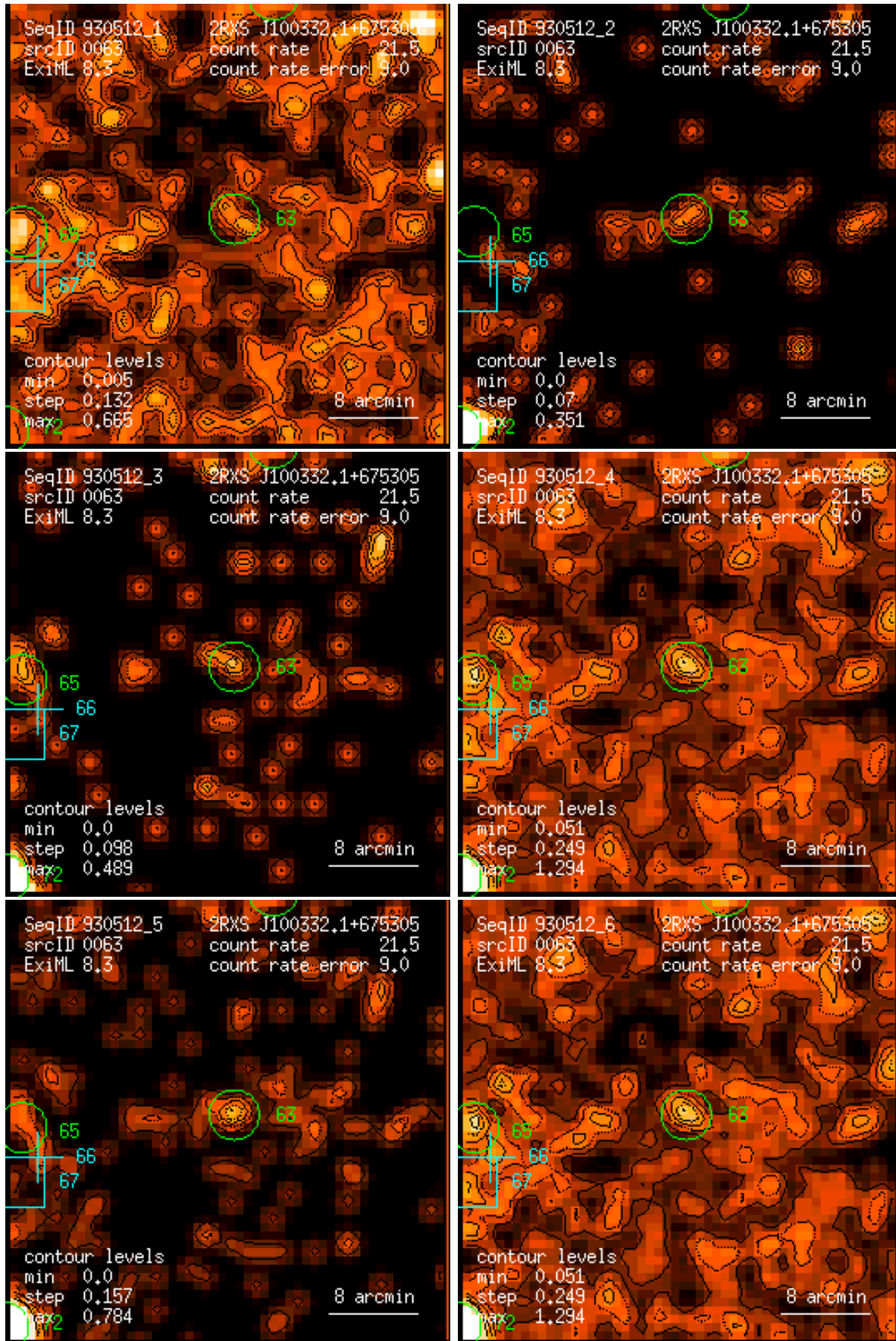
Figure 63: RASS 930512: detection 0063: band rate images, Gaussian filter: (1) PSPC channels 11 – 41, (2) 52 – 90, (3) 91 – 201, (4) 11 – 235, (5) 52 – 201, (6) 11 – 201. Broad band rates in counts/ks. Band rate contour levels in counts/ks/arcmin 2 .
