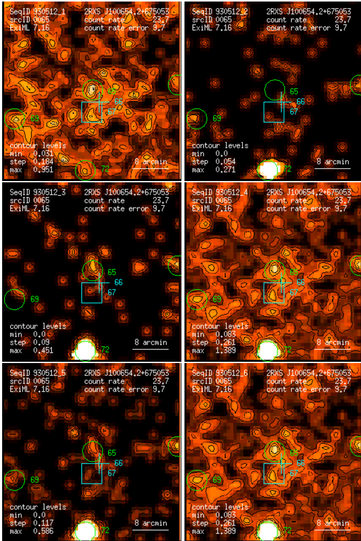
Figure 65: RASS 930512: detection 0065: band rate images, Gaussian filter: (1) PSPC channels 11 – 41, (2) 52 – 90, (3) 91 – 201, (4) 11 – 235, (5) 52 – 201, (6) 11 – 201. Broad band rates in counts/ks. Band rate contour levels in counts/ks/arcmin 2 .
