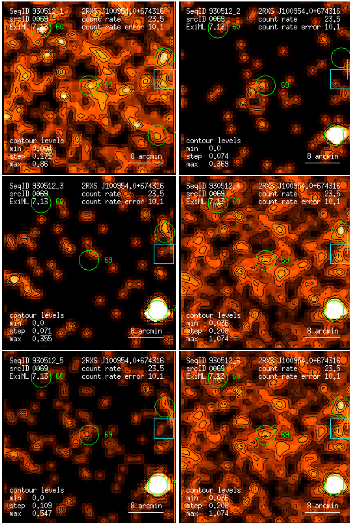
Figure 69: RASS 930512: detection 0069: band rate images, Gaussian filter: (1) PSPC channels 11 – 41, (2) 52 – 90, (3) 91 – 201, (4) 11 – 235, (5) 52 – 201, (6) 11 – 201. Broad band rates in counts/ks. Band rate contour levels in counts/ks/arcmin 2 .
