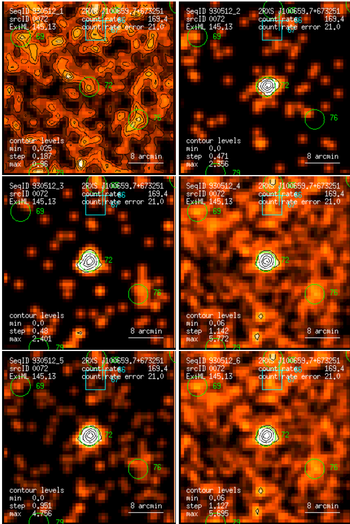
Figure 72: RASS 930512: detection 0072: band rate images, Gaussian filter: (1) PSPC channels 11 – 41, (2) 52 – 90, (3) 91 – 201, (4) 11 – 235, (5) 52 – 201, (6) 11 – 201. Broad band rates in counts/ks. Band rate contour levels in counts/ks/arcmin 2 .
