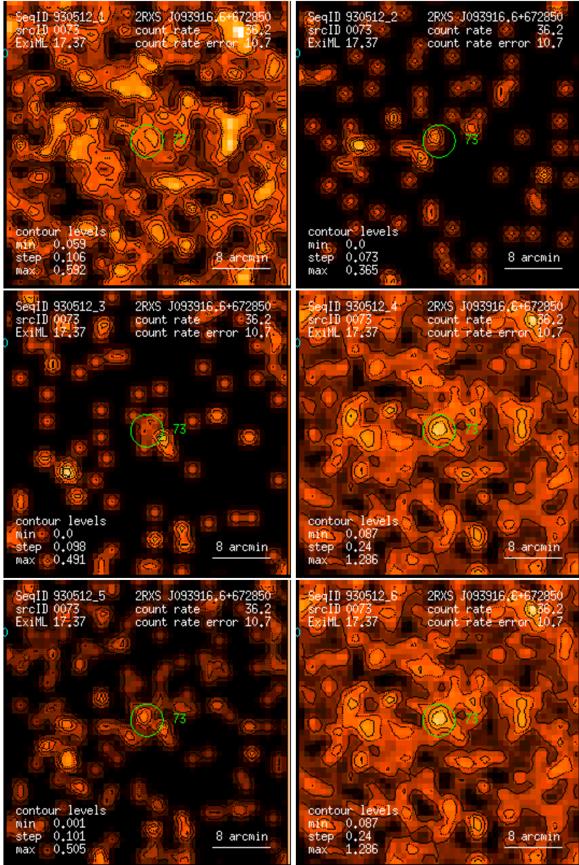
Figure 73: RASS 930512: detection 0073: band rate images, Gaussian filter: (1) PSPC channels 11 – 41, (2) 52 – 90, (3) 91 – 201, (4) 11 – 235, (5) 52 – 201, (6) 11 – 201. Broad band rates in counts/ks. Band rate contour levels in counts/ks/arcmin 2 .
